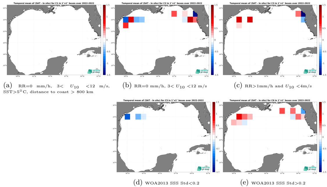
Figure 12: Temporal mean gridded over spatial boxes of size 1^{\circ}\times 1^{\circ} of \Delta\text{SSS} (SMOS SSS L2 v700 (ESA) - Sairdrone) for 5 different subdatasets corresponding to:RR=0 mm/h, 3 < U_{10} < 12 m/s, SST >5^{\circ}\text{C} , distance to coast > 800 km (a), RR=0 mm/h, 3 < U_{10} < 12 m/s (b), RR >1 mm/h and U_{10} < 4 m/s (c), WOA2013 SSS Std <0.2 (d), WOA2013 SSS Std >0.2 (e).
