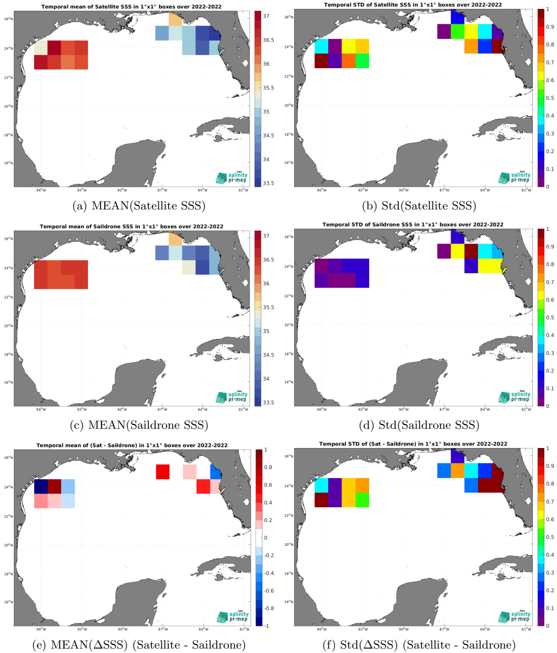
Figure 6: Temporal mean (left) and Std (right) of SSS from SMOS SSS L2 v700 (ESA) (top), Saildrone (middle), and of \Delta SSS (Satellite - Saildrone). Only match-up pairs are used to generate these maps.
