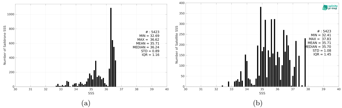
Figure 2: Histograms of SSS from Saildrone (a) and SMOS SSS L2 v700 (ESA) (b) considering all match-up pairs per bins of 0.1 over the Gulf of Mexico Pi-MEP region and for the full satellite product period.
