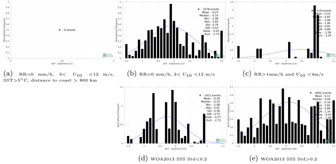
Figure 13: Normalized histogram of \Delta SSS (SMOS SSS L2 v700 (ESA) - Sairdrone) for 5 different subdatasets corresponding to: RR=0 mm/h, 3 < U_{10} < 12 m/s, SST>5°C, distance to coast > 800 km (a), RR=0 mm/h, 3 < U_{10} < 12 m/s (b), RR>1mm/h and U_{10} < 4 m/s (c), WOA2013 SSS Std<0.2 (d), WOA2013 SSS Std>0.2 (e).
