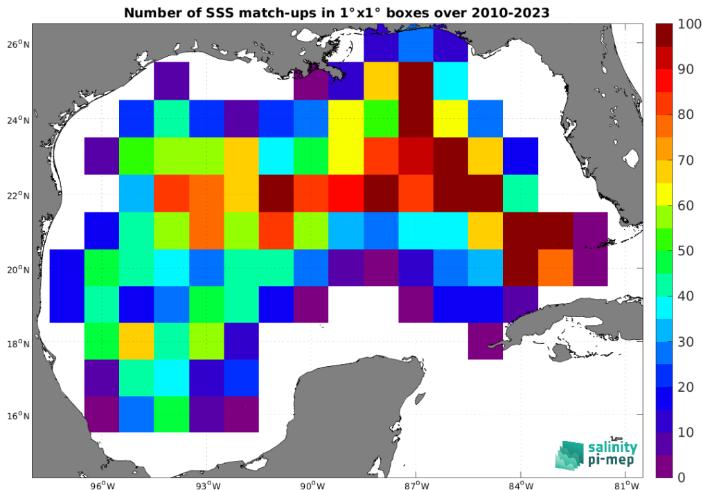
Figure 4: Number of SSS match-ups between Argo SSS and the SMOS SSS L2 v700 (ESA) SSS product for the Gulf of Mexico Pi-MEP region over 1^\circ \times 1^\circ boxes and for the full satellite product period.
