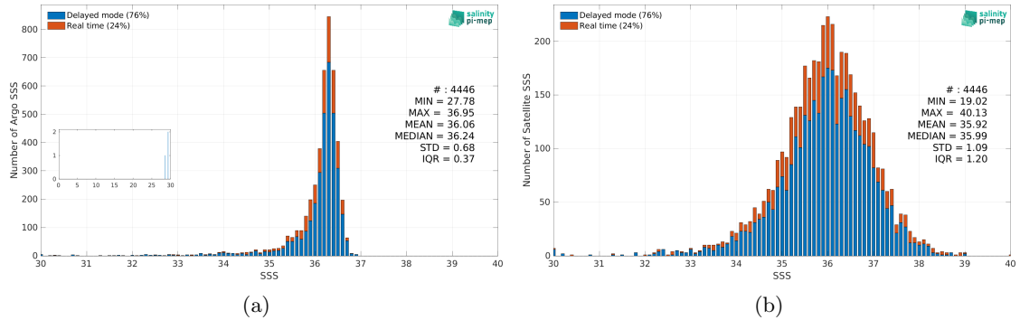
Figure 2: Histograms of SSS from Argo (a) and SMOS SSS L2 v700 (ESA) (b) considering all match-up pairs per bins of 0.1 over the Gulf of Mexico Pi-MEP region and for the full satellite product period.
