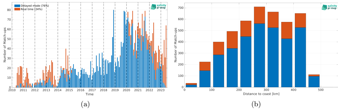
Figure 1: Number of match-ups between Argo and SMOS SSS L2 v700 (ESA) SSS as a function of time (a) and as function of the distance to coast (b) over the Gulf of Mexico Pi-MEP region and for the full satellite product period.
