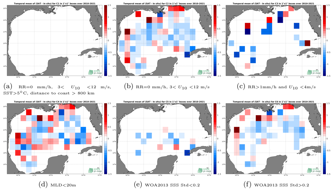
Figure 12: Temporal mean gridded over spatial boxes of size 1°x1° of \Delta SSS (SMOS SSS L2 v700 (ESA) - Argo) for 6 different subdatasets corresponding to:RR=0 mm/h, 3 < U_{10} < 12 m/s, SST>5°C, distance to coast > 800 km (a), RR=0 mm/h, 3 < U_{10} < 12 m/s (b), RR>1mm/h and U_{10} < 4 m/s (c),MLD<20m (d),WOA2013 SSS Std<0.2 (e),WOA2013 SSS Std>0.2 (f).
