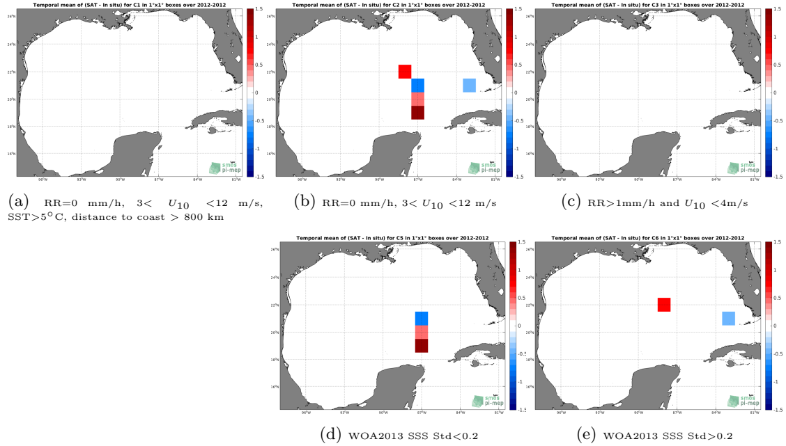
Figure 12: Temporal mean gridded over spatial boxes of size 1^{\circ}\times 1^{\circ} of \Delta SSS (SMOS SSS L2 v662 (ESA) - TSG (GOSUD-Sailing-ship)) for 5 different subdatasets corresponding to:RR=0 mm/h, 3 < U_{10} < 12 m/s, SST >5^{\circ}\text{C} , distance to coast > 800 km (a), RR=0 mm/h, 3 < U_{10} < 12 m/s (b), RR >1 mm/h and U_{10} < 4 m/s (c), WOA2013 SSS Std <0.2 (d), WOA2013 SSS Std >0.2 (e).
