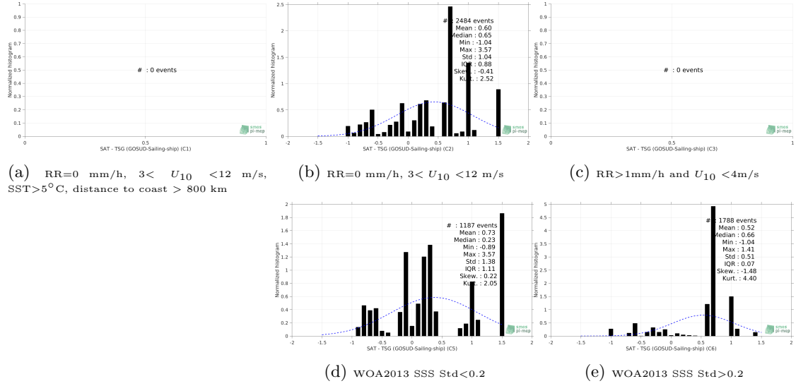
Figure 13: Normalized histogram of \Delta\text{SSS} (SMOS SSS L2 v662 (ESA) - TSG (GOSUD-Sailing-ship)) for 5 different subdatasets corresponding to: RR=0 mm/h, 3 < U_{10} < 12 m/s, SST > 5^{\circ}\text{C} , distance to coast > 800 km (a), RR=0 mm/h, 3 < U_{10} < 12 m/s (b), RR > 1\text{mm/h} and U_{10} < 4\text{m/s} (c), WOA2013 SSS Std < 0.2 (d), WOA2013 SSS Std > 0.2 (e).
