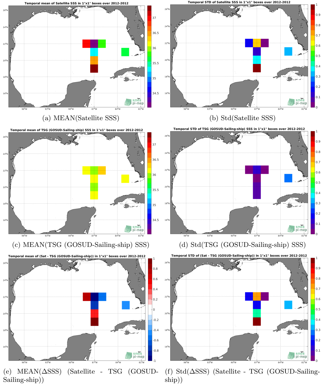
Figure 6: Temporal mean (left) and Std (right) of SSS from SMOS SSS L2 v662 (ESA) (top), TSG (GOSUD-Sailing-ship) (middle), and of \Delta SSS (Satellite - TSG (GOSUD-Sailing-ship)). Only match-up pairs are used to generate these maps.
