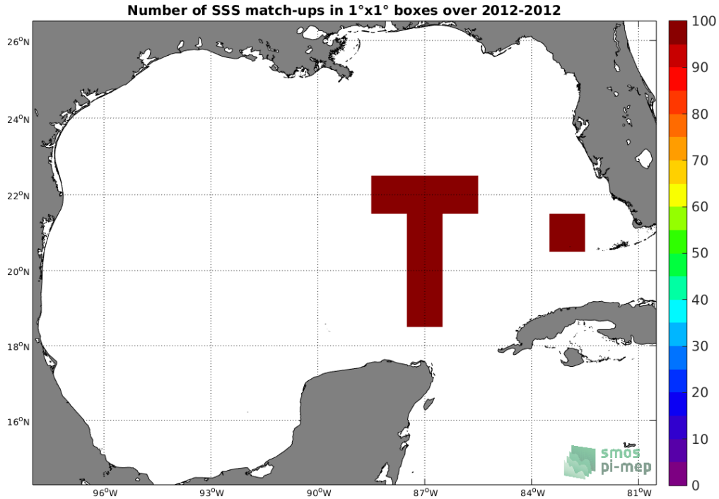
Figure 4: Number of SSS match-ups between TSG (GOSUD-Sailing-ship) SSS and the SMOS SSS L2 v662 (ESA) SSS product for the Gulf of Mexico Pi-MEP region over 1°x1° boxes and for the full satellite product period.
