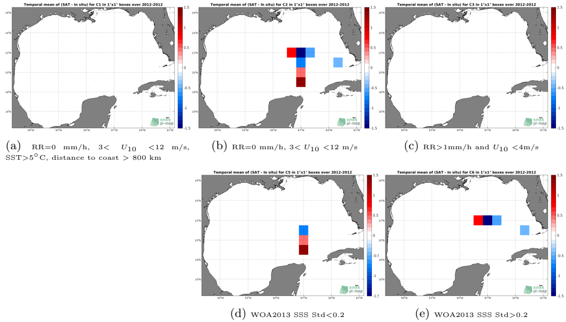
Figure 12: Temporal mean gridded over spatial boxes of size 1^\circ \times 1^\circ of \Delta SSS (SMOS SSS L2 v662 (ESA) - TSG (GOSUD-Sailing-ship)) for 5 different subdatasets corresponding to: RR=0 mm/h, 3 < U_{10} < 12 m/s, SST >5^\circ\text{C} , distance to coast > 800 km (a), RR=0 mm/h, 3 < U_{10} < 12 m/s (b), RR >1 mm/h and U_{10} < 4 m/s (c), WOA2013 SSS Std <0.2 (d), WOA2013 SSS Std >0.2 (e).
