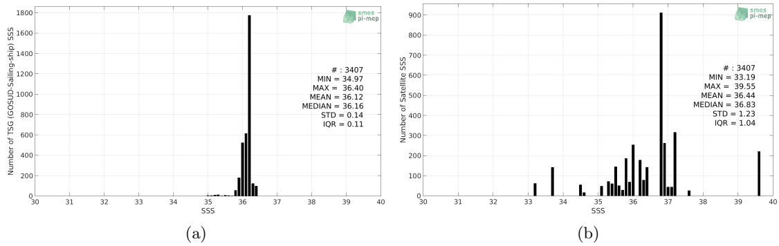
Figure 2: Histograms of SSS from TSG (GOSUD-Sailing-ship) (a) and SMOS SSS L2 v662 (ESA) (b) considering all match-up pairs per bins of 0.1 over the Gulf of Mexico Pi-MEP region and for the full satellite product period.
