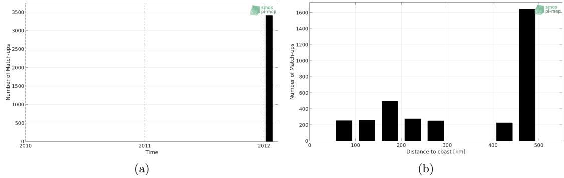
Figure 1: Number of match-ups between TSG (GOSUD-Sailing-ship) and SMOS SSS L2 v662 (ESA) SSS as a function of time (a) and as function of the distance to coast (b) over the Gulf of Mexico Pi-MEP region and for the full satellite product period.
