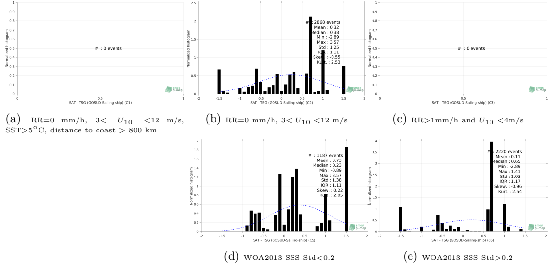
Figure 13: Normalized histogram of \Delta\text{SSS} (SMOS SSS L2 v662 (ESA) - TSG (GOSUD-Sailing-ship)) for 5 different subdatasets corresponding to: RR=0 mm/h, 3 < U_{10} < 12 m/s, SST > 5^\circ\text{C} , distance to coast > 800 km (a), RR=0 mm/h, 3 < U_{10} < 12 m/s (b), RR > 1\text{mm/h} and U_{10} < 4\text{m/s} (c), WOA2013 SSS Std < 0.2 (d), WOA2013 SSS Std > 0.2 (e).
