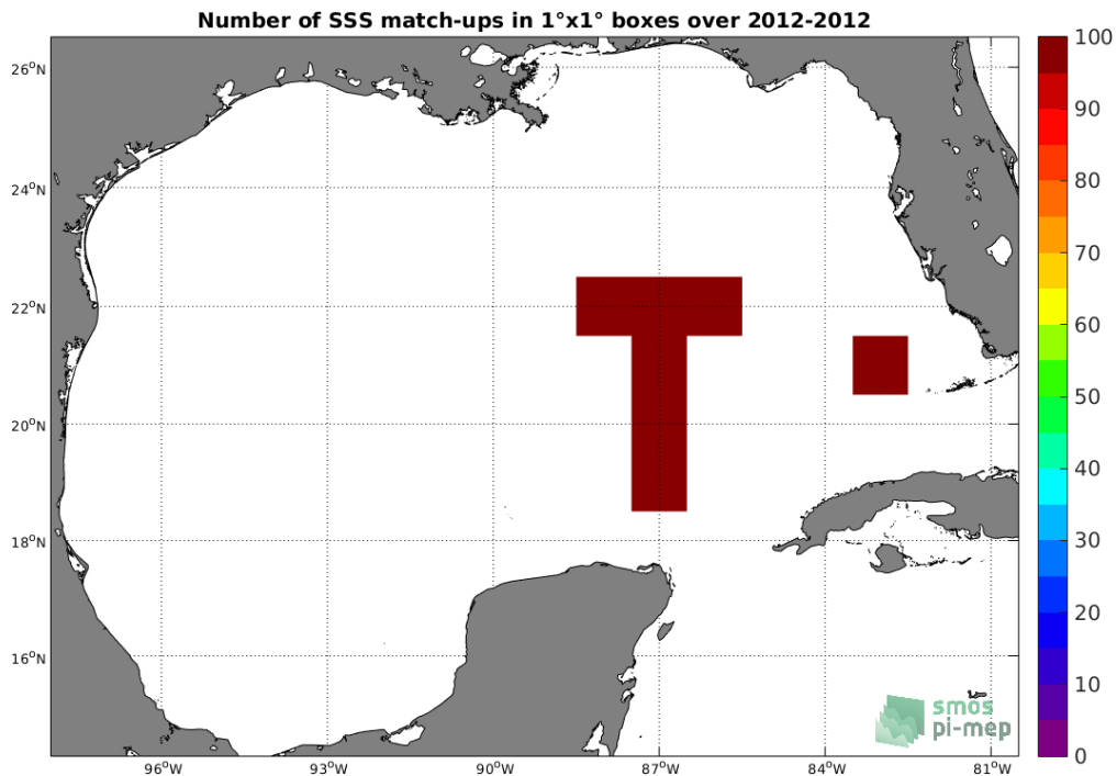
Figure 4: Number of SSS match-ups between TSG-GOSUD-Sailing-ship SSS and the SMOS L2 v662 (ESA) SSS product for the Gulf of Mexico Pi-MEP region over 1°x1° boxes and for the full satellite product period.
