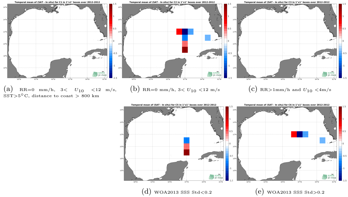
Figure 12: Temporal mean gridded over spatial boxes of size 1^\circ \times 1^\circ of \Delta SSS (SMOS L2 v662 (ESA) - TSG-GOSUD-Sailing-ship) for 5 different subdatasets corresponding to: RR=0 mm/h, 3 < U_{10} < 12 m/s, SST >5^\circ\text{C} , distance to coast > 800 km (a), RR=0 mm/h, 3 < U_{10} < 12 m/s (b), RR >1 mm/h and U_{10} < 4 m/s (c), WOA2013 SSS Std <0.2 (d), WOA2013 SSS Std >0.2 (e).
