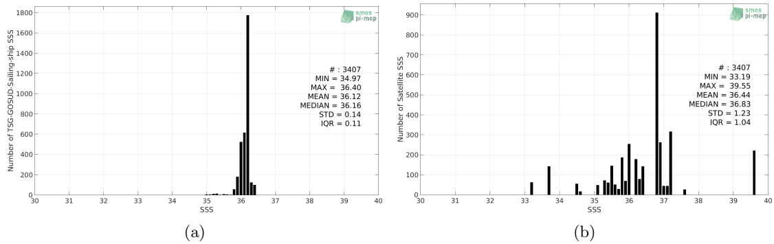
Figure 2: Histograms of SSS from TSG-GOSUD-Sailing-ship (a) and SMOS L2 v662 (ESA) (b) considering all match-up pairs per bins of 0.1 over the Gulf of Mexico Pi-MEP region and for the full satellite product period.
