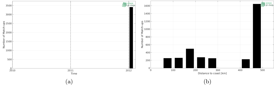
Figure 1: Number of match-ups between TSG-GOSUD-Sailing-ship and SMOS L2 v662 (ESA) SSS as a function of time (a) and as function of the distance to coast (b) over the Gulf of Mexico Pi-MEP region and for the full satellite product period.
