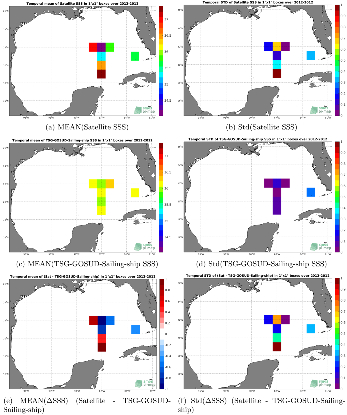
Figure 6: Temporal mean (left) and Std (right) of SSS from SMOS L2 v662 (ESA) (top), TSG-GOSUD-Sailing-ship (middle), and of \Delta SSS (Satellite - TSG-GOSUD-Sailing-ship). Only match-up pairs are used to generate these maps.
