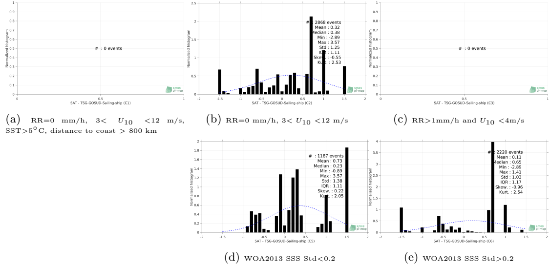
Figure 13: Normalized histogram of \Delta SSS (SMOS L2 v662 (ESA) - TSG-GOSUD-Sailing-ship) for 5 different subdatasets corresponding to: RR=0 mm/h, 3 < U_{10} < 12 m/s, SST>5°C, distance to coast > 800 km (a), RR=0 mm/h, 3 < U_{10} < 12 m/s (b), RR>1 mm/h and U_{10} < 4 m/s (c), WOA2013 SSS Std<0.2 (d), WOA2013 SSS Std>0.2 (e).
