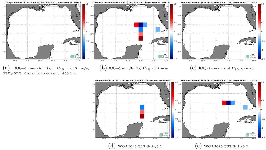
Figure 12: Temporal mean gridded over spatial boxes of size 1^\circ \times 1^\circ of \Delta SSS (SMOS-L2-DPGS-v662 - TSG-GOSUD-Sailing-ship) for 5 different subdatasets corresponding to: RR=0 mm/h, 3 < U_{10} < 12 m/s, SST > 5^\circ\text{C} , distance to coast > 800 km (a), RR=0 mm/h, 3 < U_{10} < 12 m/s (b), RR > 1 mm/h and U_{10} < 4 m/s (c), WOA2013 SSS Std < 0.2 (d), WOA2013 SSS Std > 0.2 (e).
