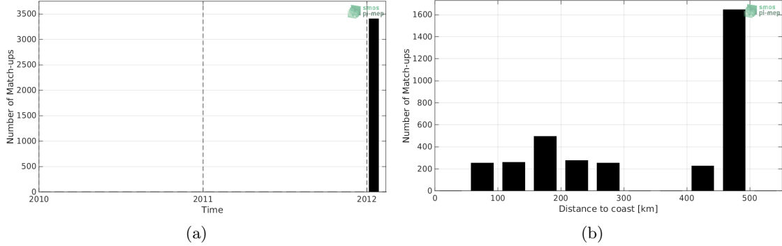
Figure 1: Number of match-ups between TSG-GOSUD-Sailing-ship and SMOS-L2-DPGS-v662 SSS as a function of time (a) and as function of the distance to coast (b) over the Gulf of Mexico Pi-MEP region and for the full satellite product period.
