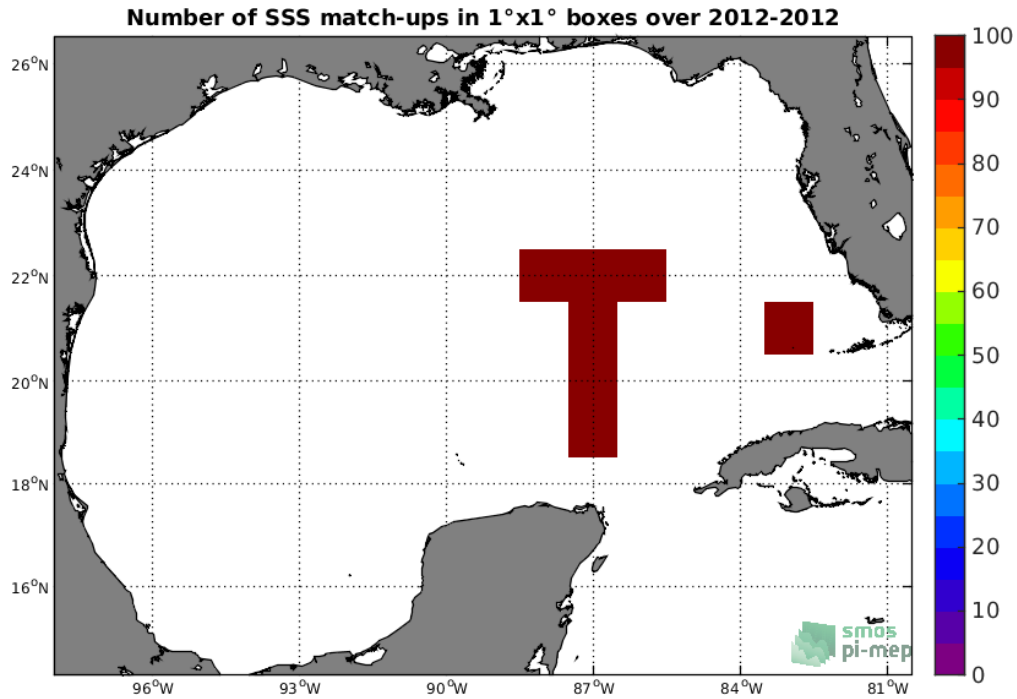
Figure 4: Number of SSS match-ups between TSG-GOSUD-Sailing-ship SSS and the SMOS-L2-DPGS-v662 SSS product for the Gulf of Mexico Pi-MEP region over 1°x1° boxes and for the full satellite product period.
