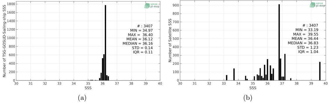
Figure 2: Histograms of SSS from TSG-GOSUD-Sailing-ship (a) and SMOS-L2-DPGS-v662 (b) considering all match-up pairs per bins of 0.1 over the Gulf of Mexico Pi-MEP region and for the full satellite product period.
