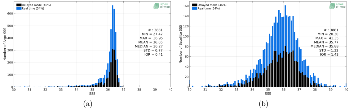
Figure 2: Histograms of SSS from Argo (a) and SMOS SSS L2 v662 (ESA) (b) considering all match-up pairs per bins of 0.1 over the Gulf of Mexico Pi-MEP region and for the full satellite product period.
