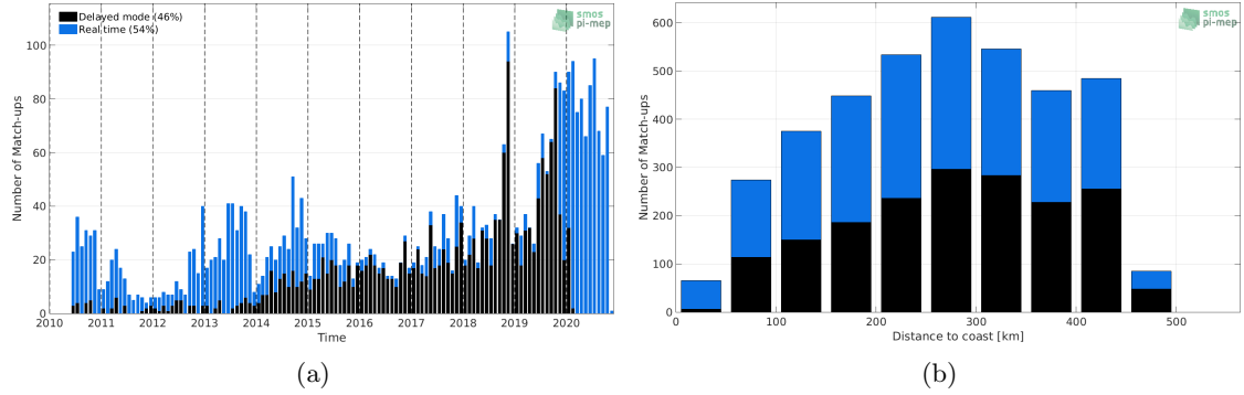
Figure 1: Number of match-ups between Argo and SMOS SSS L2 v662 (ESA) SSS as a function of time (a) and as function of the distance to coast (b) over the Gulf of Mexico Pi-MEP region and for the full satellite product period.
