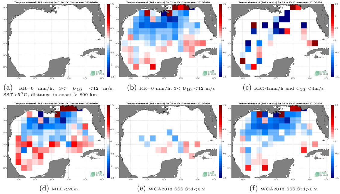
Figure 12: Temporal mean gridded over spatial boxes of size 1^\circ \times 1^\circ of \Delta SSS (SMOS SSS L2 v662 (ESA) - Argo) for 6 different subdatasets corresponding to:RR=0 mm/h, 3 < U_{10} < 12 m/s, SST >5^\circ\text{C} , distance to coast > 800 km (a), RR=0 mm/h, 3 < U_{10} < 12 m/s (b), RR >1 mm/h and U_{10} < 4 m/s (c),MLD <20 m (d),WOA2013 SSS Std <0.2 (e),WOA2013 SSS Std >0.2 (f).
