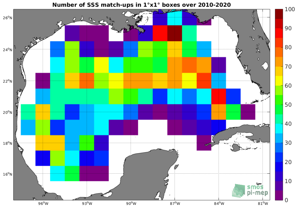
Figure 4: Number of SSS match-ups between Argo SSS and the SMOS SSS L2 v662 (ESA) SSS product for the Gulf of Mexico Pi-MEP region over 1^\circ \times 1^\circ boxes and for the full satellite product period.
