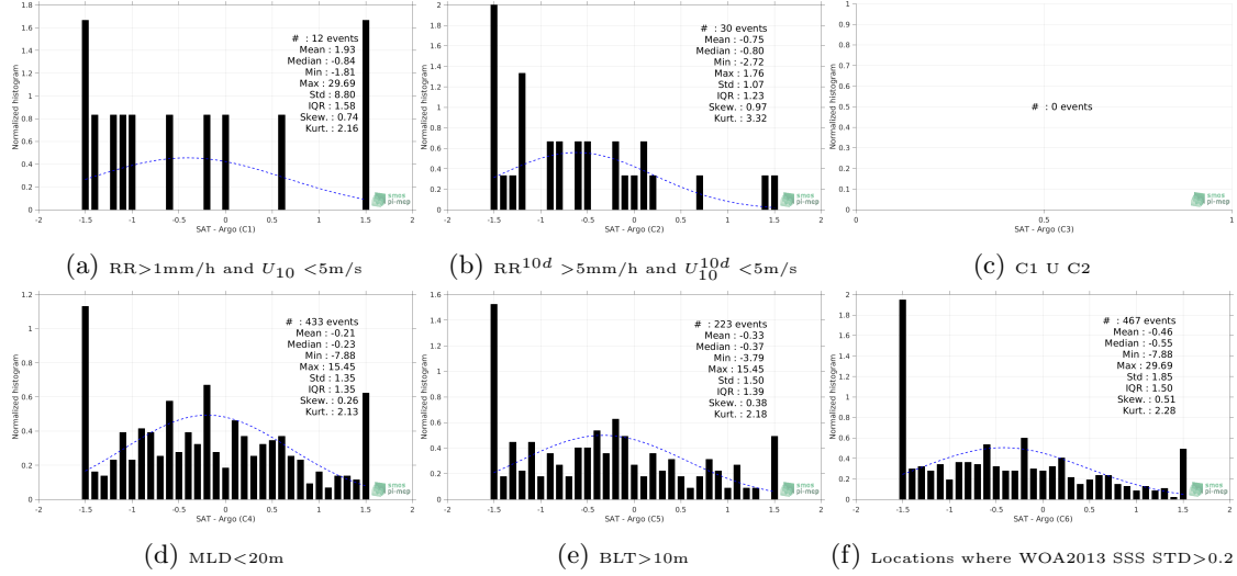
Figure 13: Normalized histogram of \Delta\text{SSS} (SMOS-L2-DPGS-v662 - Argo) for 6 different sub-datasets corresponding to: RR > 1\text{mm/h} and U_{10} < 5\text{m/s} (a), RR^{10d} > 5\text{mm/h} and U_{10}^{10d} < 5\text{m/s} (b), C1 U C2 (c), MLD < 20\text{m} (d), BLT > 10\text{m} (e), Locations where WOA2013 SSS STD > 0.2 (f).
