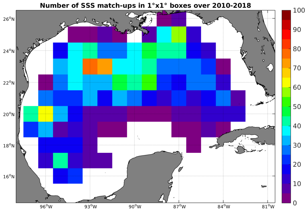
Figure 4: Number of SSS match-ups between Argo SSS and the SMOS-L2-DPGS-v662 SSS product for the Gulf of Mexico Pi-MEP region over 1^\circ \times 1^\circ boxes and for the full satellite product period.
