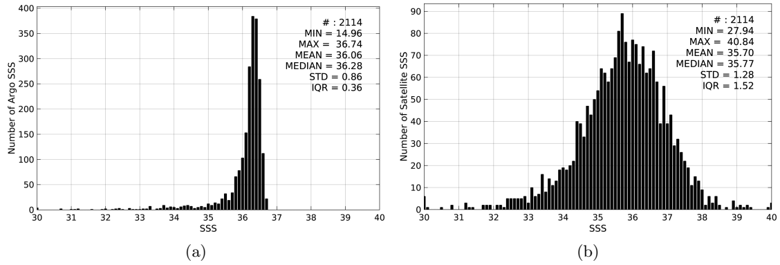
Figure 2: Histograms of SSS from Argo (a) and SMOS-L2-DPGS-v662 (b) considering all match-up pairs per bins of 0.1 over the Gulf of Mexico Pi-MEP region and for the full satellite product period.
