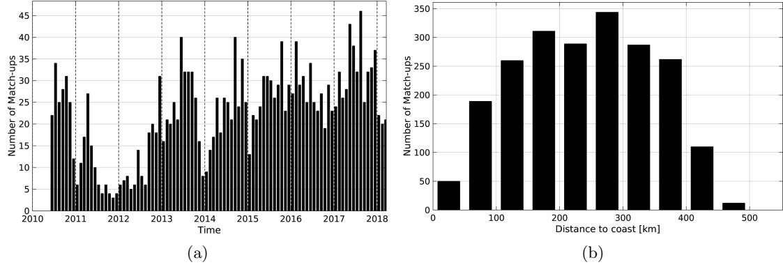
Figure 1: Number of match-ups between Argo and SMOS-L2-DPGS-v662 SSS as a function of time (a) and as function of the distance to coast (b) over the Gulf of Mexico Pi-MEP region and for the full satellite product period.
