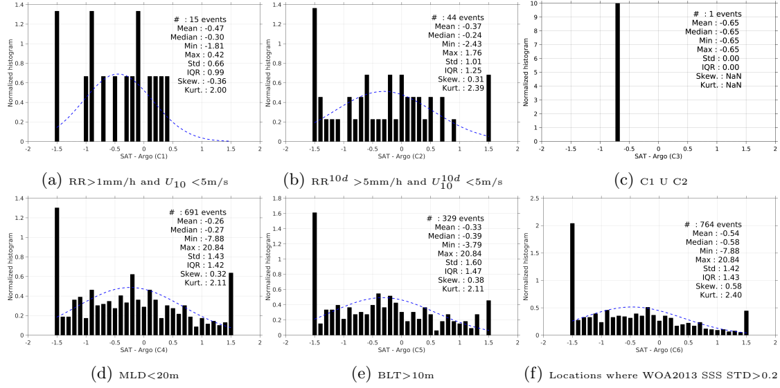
Figure 13: Normalized histogram of \Delta SSS (SMOS-L2-DPGS-v662 - Argo) for 6 different sub-datasets corresponding to: RR > 1\text{mm/h} and U_{10} < 5\text{m/s} (a), RR^{10d} > 5\text{mm/h} and U_{10}^{10d} < 5\text{m/s} (b), C1 U C2 (c), MLD < 20\text{m} (d), BLT > 10\text{m} (e), Locations where WOA2013 SSS STD > 0.2 (f).
