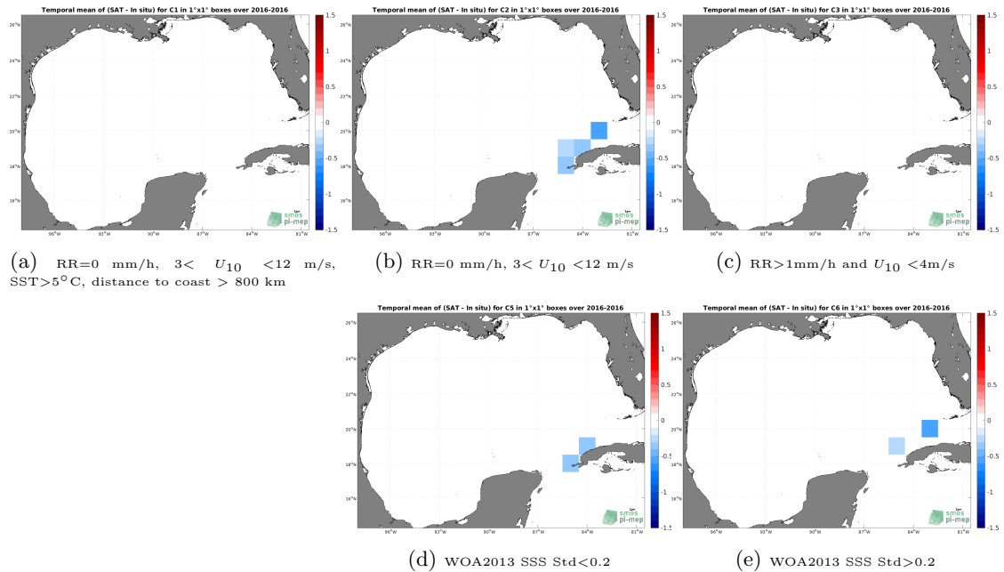
Figure 12: Temporal mean gridded over spatial boxes of size 1^{\circ}\times 1^{\circ} of \Delta\text{SSS} (SMAP SSS L4 OI v1 - 7 Days (IPRC) - TSG (LEGOS-DM)) for 5 different subdatasets corresponding to:RR=0 mm/h, 3 < U_{10} < 12 m/s, SST > 5^{\circ}\text{C} , distance to coast > 800 km (a), RR=0 mm/h, 3 < U_{10} < 12 m/s (b), RR > 1 mm/h and U_{10} < 4 m/s (c), WOA2013 SSS Std < 0.2 (d), WOA2013 SSS Std > 0.2 (e).
