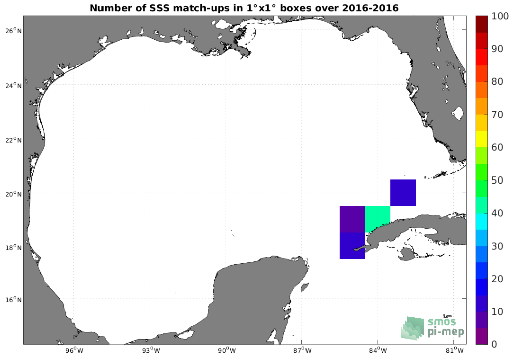
Figure 4: Number of SSS match-ups between TSG (LEGOS-DM) SSS and the SMAP SSS L4 OI v1 - 7 Days (IPRC) SSS product for the Gulf of Mexico Pi-MEP region over 1°x1° boxes and for the full satellite product period.
