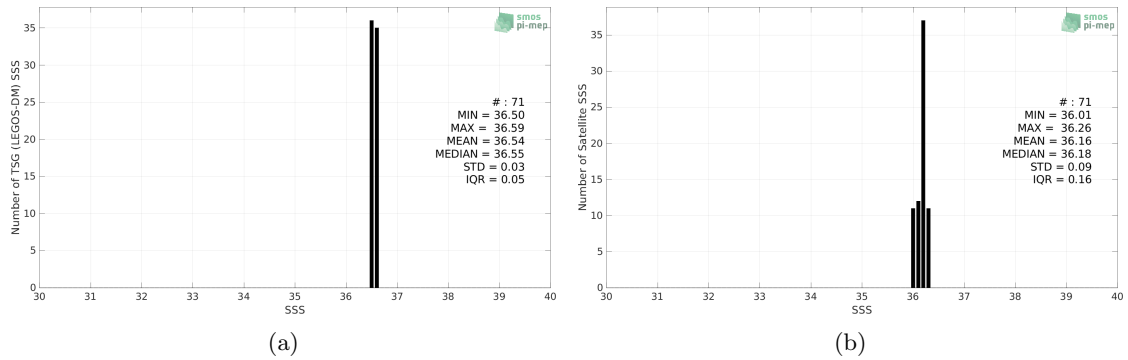
Figure 2: Histograms of SSS from TSG (LEGOS-DM) (a) and SMAP SSS L4 OI v1 - 7 Days (IPRC) (b) considering all match-up pairs per bins of 0.1 over the Gulf of Mexico Pi-MEP region and for the full satellite product period.
