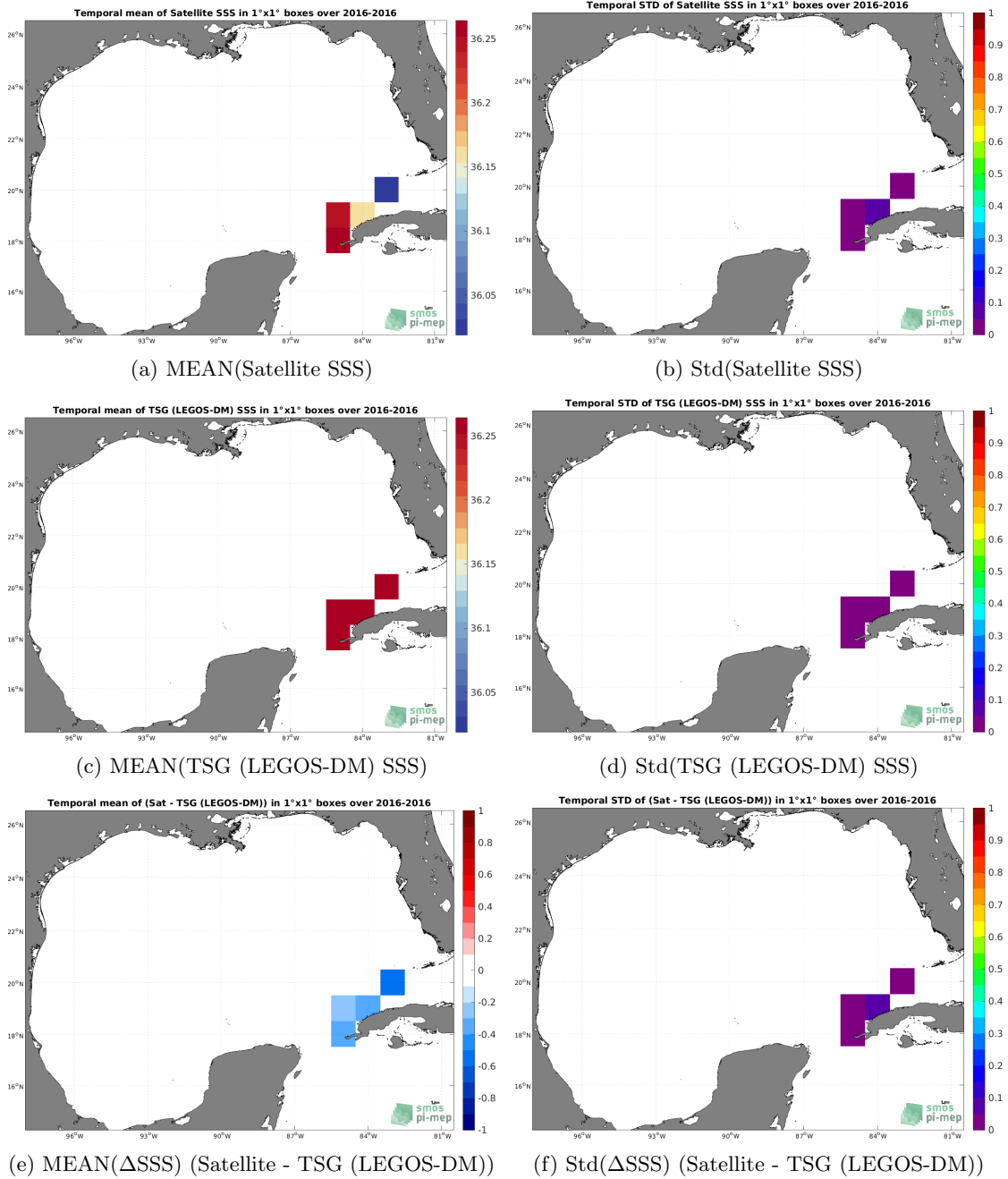
Figure 6: Temporal mean (left) and Std (right) of SSS from SMAP SSS L4 OI v1 - 7 Days (IPRC) (top), TSG (LEGOS-DM) (middle), and of \Delta SSS (Satellite - TSG (LEGOS-DM)). Only match-up pairs are used to generate these maps.
