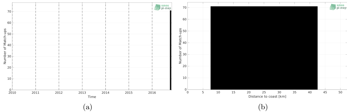
Figure 1: Number of match-ups between TSG (LEGOS-DM) and SMAP SSS L4 OI v1 - 7 Days (IPRC) SSS as a function of time (a) and as function of the distance to coast (b) over the Gulf of Mexico Pi-MEP region and for the full satellite product period.
