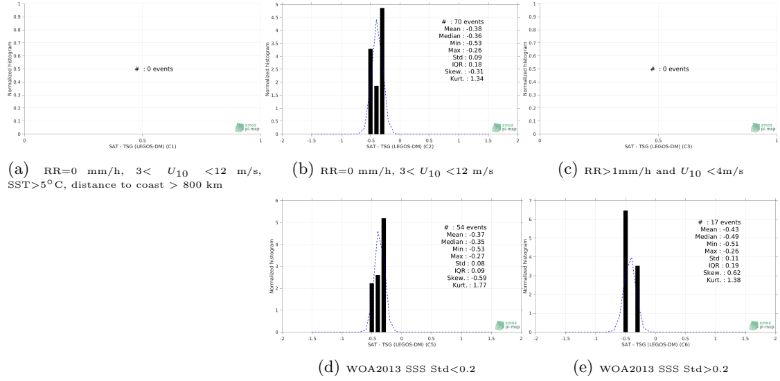
Figure 13: Normalized histogram of \Delta\text{SSS} (SMAP SSS L4 OI v1 - 7 Days (IPRC) - TSG (LEGOS-DM)) for 5 different subdatasets corresponding to: RR=0 mm/h, 3 < U_{10} < 12 m/s, SST > 5^\circ\text{C} , distance to coast > 800 km (a), RR=0 mm/h, 3 < U_{10} < 12 m/s (b), RR > 1\text{mm/h} and U_{10} < 4\text{m/s} (c), WOA2013 SSS Std < 0.2 (d), WOA2013 SSS Std > 0.2 (e).
