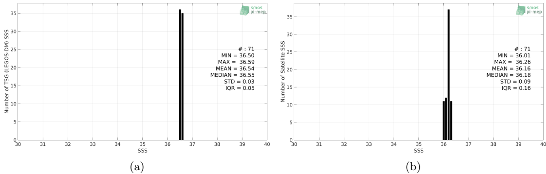
Figure 2: Histograms of SSS from TSG (LEGOS-DM) (a) and SMAP SSS L4 OI v1 - 7day (IPRC) (b) considering all match-up pairs per bins of 0.1 over the Gulf of Mexico Pi-MEP region and for the full satellite product period.
