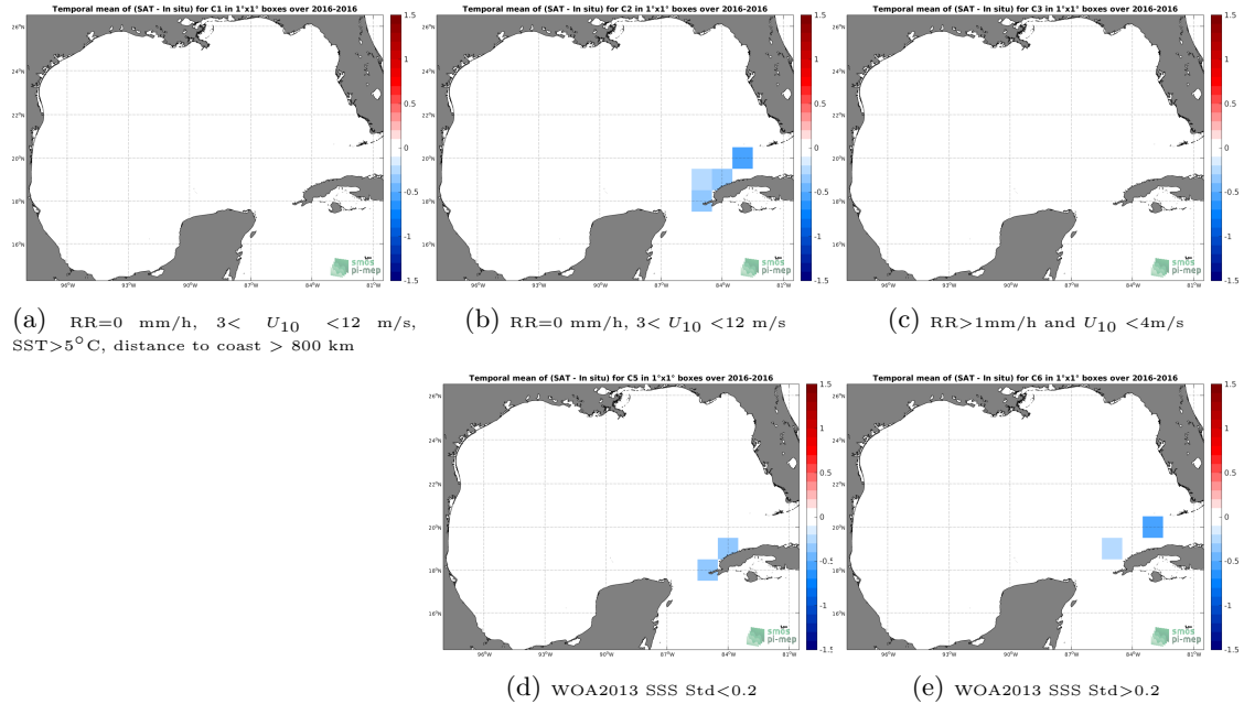
Figure 12: Temporal mean gridded over spatial boxes of size 1^{\circ}\times 1^{\circ} of \Delta\text{SSS} (SMAP SSS L4 OI v1 - 7day (IPRC) - TSG (LEGOS-DM)) for 5 different subdatasets corresponding to:RR=0 mm/h, 3 < U_{10} < 12 m/s, SST >5^{\circ}\text{C} , distance to coast > 800 km (a), RR=0 mm/h, 3 < U_{10} < 12 m/s (b), RR >1 mm/h and U_{10} < 4 m/s (c), WOA2013 SSS Std <0.2 (d), WOA2013 SSS Std >0.2 (e).
