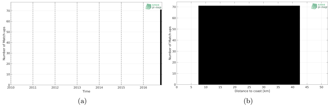
Figure 1: Number of match-ups between TSG (LEGOS-DM) and SMAP SSS L4 OI v1 - 7day (IPRC) SSS as a function of time (a) and as function of the distance to coast (b) over the Gulf of Mexico Pi-MEP region and for the full satellite product period.
