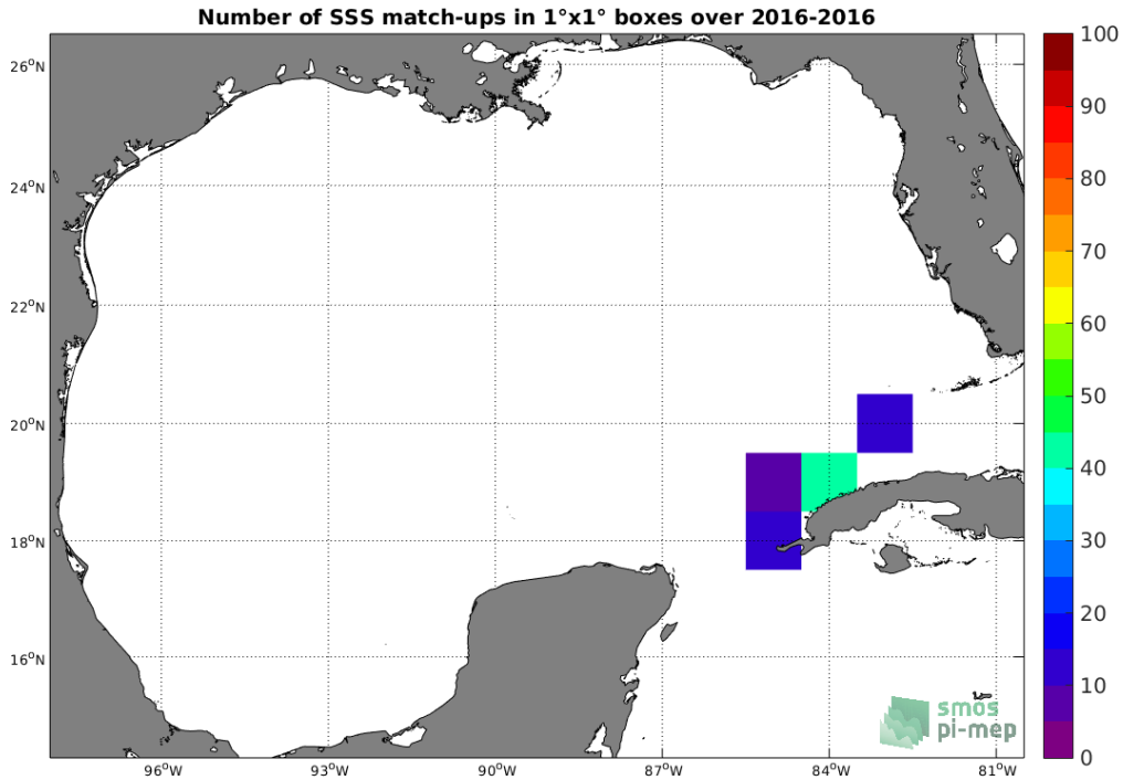
Figure 4: Number of SSS match-ups between TSG (LEGOS-DM) SSS and the SMAP SSS L4 OI v1 - 7day (IPRC) SSS product for the Gulf of Mexico Pi-MEP region over 1°x1° boxes and for the full satellite product period.
