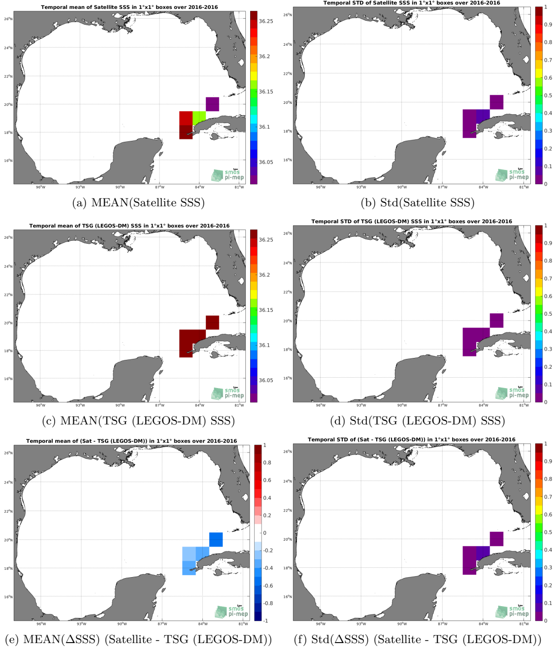
Figure 6: Temporal mean (left) and Std (right) of SSS from SMAP SSS L4 OI v1 - 7day (IPRC) (top), TSG (LEGOS-DM) (middle), and of \Delta SSS (Satellite - TSG (LEGOS-DM)). Only match-up pairs are used to generate these maps.
