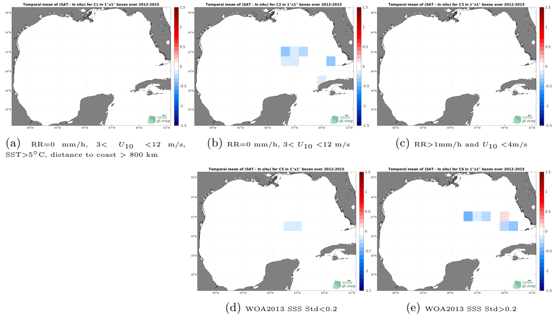
Figure 12: Temporal mean gridded over spatial boxes of size 1^{\circ}\times 1^{\circ} of \Delta SSS (SMAP SSS L4 OI v1 - 7 Days (IPRC) - TSG (GOSUD-Sailing-ship)) for 5 different subdatasets corresponding to:RR=0 mm/h, 3 < U_{10} < 12 m/s, SST >5^{\circ}\text{C} , distance to coast > 800 km (a), RR=0 mm/h, 3 < U_{10} < 12 m/s (b), RR >1 mm/h and U_{10} < 4 m/s (c), WOA2013 SSS Std <0.2 (d), WOA2013 SSS Std >0.2 (e).
