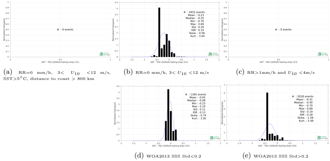
Figure 13: Normalized histogram of \Delta SSS (SMAP SSS L4 OI v1 - 7 Days (IPRC) - TSG (GOSUD-Sailing-ship)) for 5 different subdatasets corresponding to: RR=0 mm/h, 3 < U_{10} < 12 m/s, SST > 5°C, distance to coast > 800 km (a), RR=0 mm/h, 3 < U_{10} < 12 m/s (b), RR > 1mm/h and U_{10} < 4 m/s (c), WOA2013 SSS Std < 0.2 (d), WOA2013 SSS Std > 0.2 (e).
