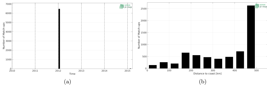
Figure 1: Number of match-ups between TSG (GOSUD-Sailing-ship) and SMAP SSS L4 OI v1 - 7 Days (IPRC) SSS as a function of time (a) and as function of the distance to coast (b) over the Gulf of Mexico Pi-MEP region and for the full satellite product period.
