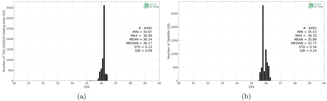
Figure 2: Histograms of SSS from TSG (GOSUD-Sailing-ship) (a) and SMAP SSS L4 OI v1 - 7 Days (IPRC) (b) considering all match-up pairs per bins of 0.1 over the Gulf of Mexico Pi-MEP region and for the full satellite product period.
