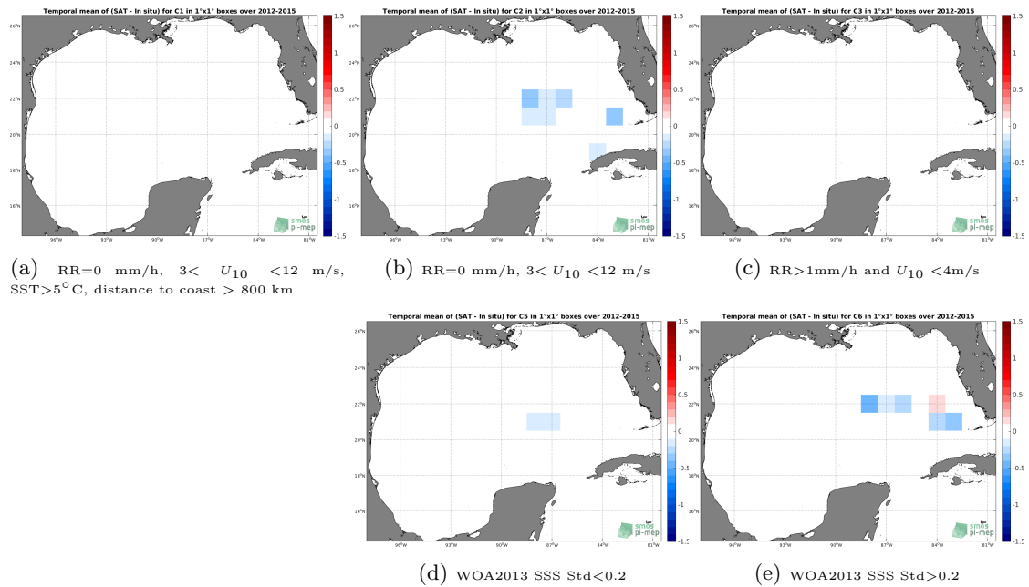
Figure 12: Temporal mean gridded over spatial boxes of size 1^\circ \times 1^\circ of \Delta SSS (SMAP SSS L4 OI v1 - 7 Days (IPRC) - TSG (GOSUD-Sailing-ship)) for 5 different subdatasets corresponding to:RR=0 mm/h, 3 < U_{10} < 12 m/s, SST >5^\circ\text{C} , distance to coast > 800 km (a), RR=0 mm/h, 3 < U_{10} < 12 m/s (b), RR >1 mm/h and U_{10} < 4 m/s (c), WOA2013 SSS Std <0.2 (d), WOA2013 SSS Std >0.2 (e).
