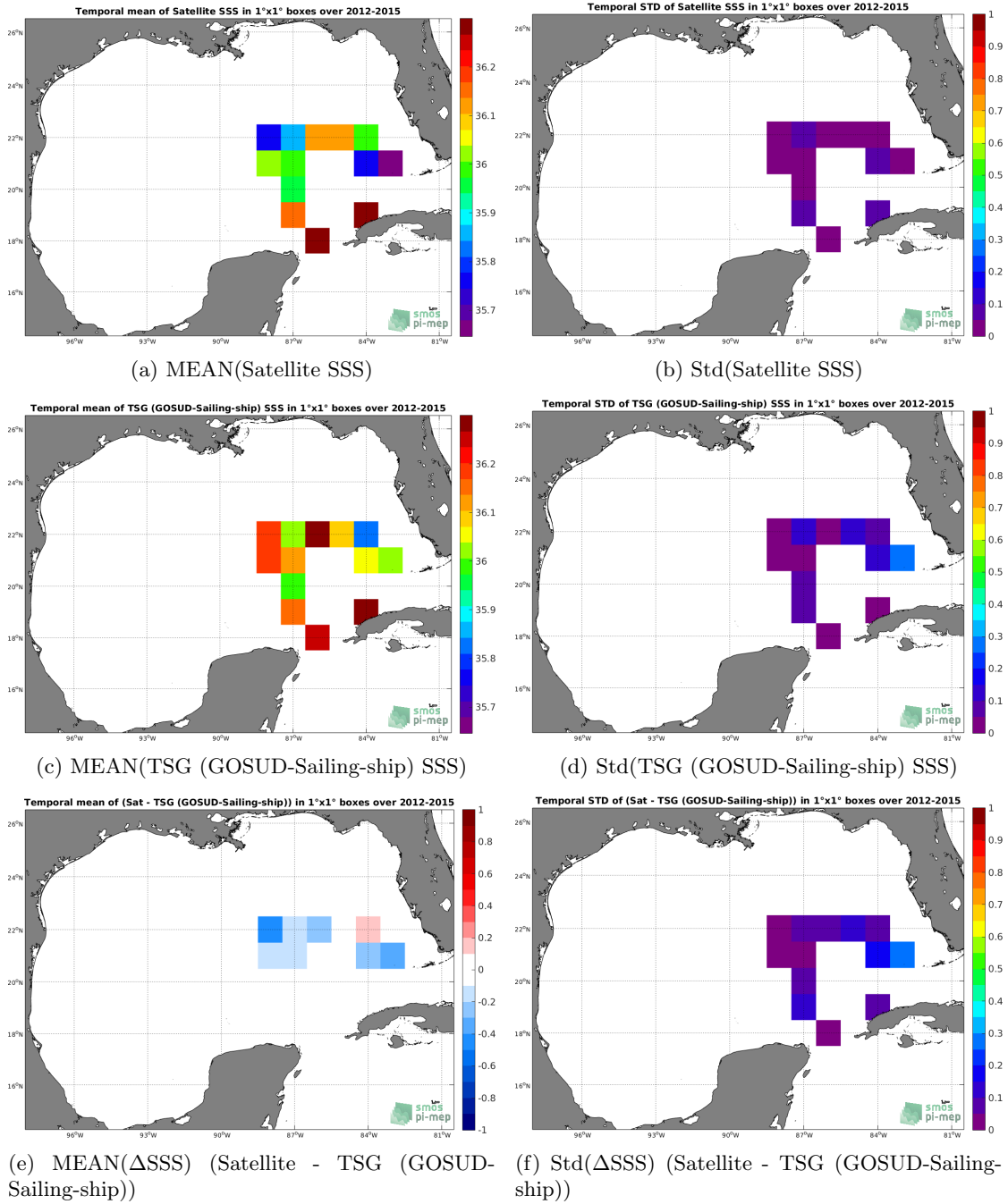
Figure 6: Temporal mean (left) and Std (right) of SSS from SMAP SSS L4 OI v1 - 7day (IPRC) (top), TSG (GOSUD-Sailing-ship) (middle), and of \Delta SSS (Satellite - TSG (GOSUD-Sailing-ship)). Only match-up pairs are used to generate these maps.
