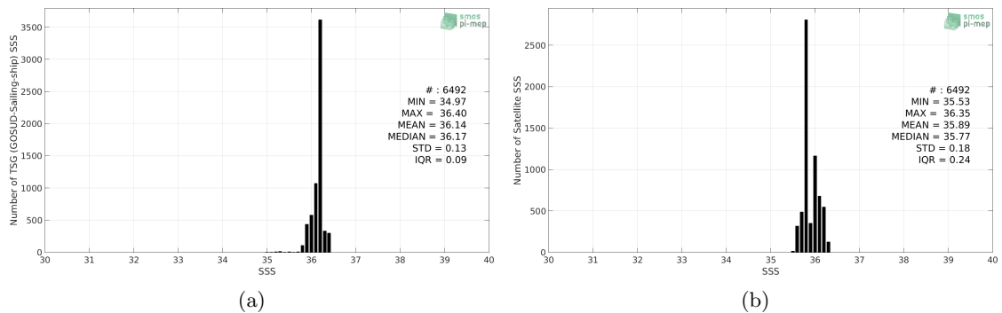
Figure 2: Histograms of SSS from TSG (GOSUD-Sailing-ship) (a) and SMAP SSS L4 OI v1 - 7day (IPRC) (b) considering all match-up pairs per bins of 0.1 over the Gulf of Mexico Pi-MEP region and for the full satellite product period.
