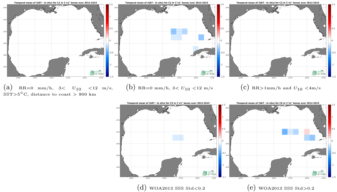
Figure 12: Temporal mean gridded over spatial boxes of size 1^\circ \times 1^\circ of \Delta SSS (SMAP SSS L4 OI v1 - 7day (IPRC) - TSG (GOSUD-Sailing-ship)) for 5 different subdatasets corresponding to:RR=0 mm/h, 3 < U_{10} < 12 m/s, SST >5^\circ\text{C} , distance to coast > 800 km (a), RR=0 mm/h, 3 < U_{10} < 12 m/s (b), RR >1 mm/h and U_{10} < 4 m/s (c), WOA2013 SSS Std <0.2 (d), WOA2013 SSS Std >0.2 (e).
