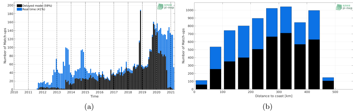
Figure 1: Number of match-ups between Argo and SMAP SSS L4 OI v1 - 7 Days (IPRC) SSS as a function of time (a) and as function of the distance to coast (b) over the Gulf of Mexico Pi-MEP region and for the full satellite product period.
