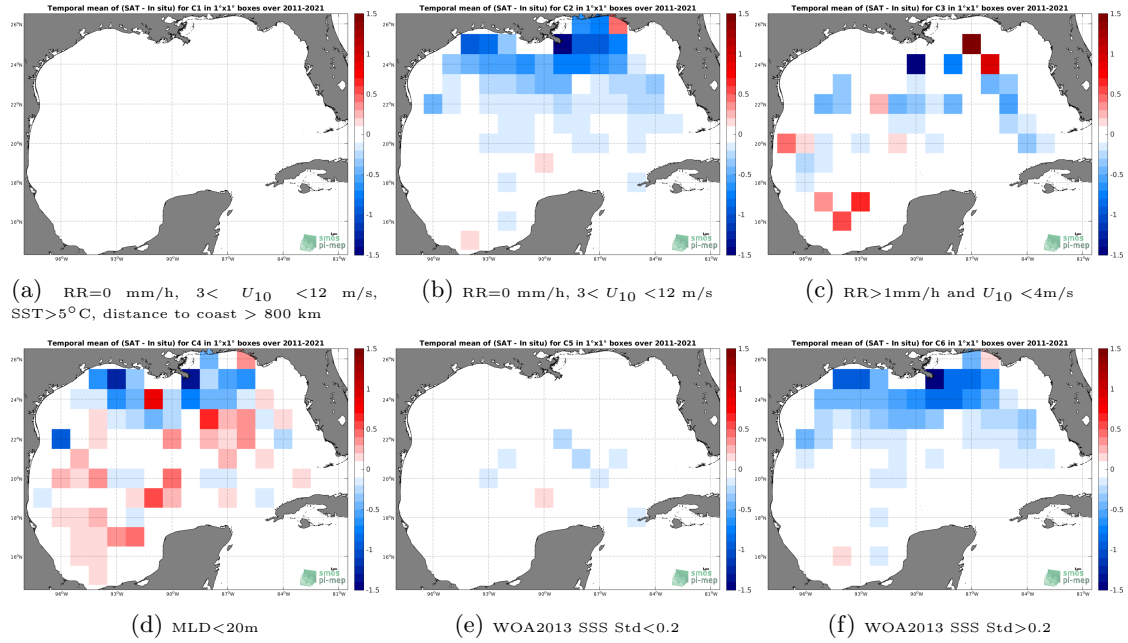
Figure 12: Temporal mean gridded over spatial boxes of size 1^\circ \times 1^\circ of \Delta SSS (SMAP SSS L4 OI v1 - 7 Days (IPRC) - Argo) for 6 different subdatasets corresponding to:RR=0 mm/h, 3 < U_{10} < 12 m/s, SST >5^\circ\text{C} , distance to coast > 800 km (a), RR=0 mm/h, 3 < U_{10} < 12 m/s (b), RR >1 mm/h and U_{10} < 4 m/s (c),MLD <20 m (d),WOA2013 SSS Std <0.2 (e),WOA2013 SSS Std >0.2 (f).
