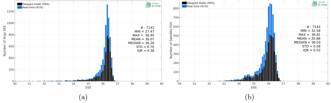
Figure 2: Histograms of SSS from Argo (a) and SMAP SSS L4 OI v1 - 7day (IPRC) (b) considering all match-up pairs per bins of 0.1 over the Gulf of Mexico Pi-MEP region and for the full satellite product period.
