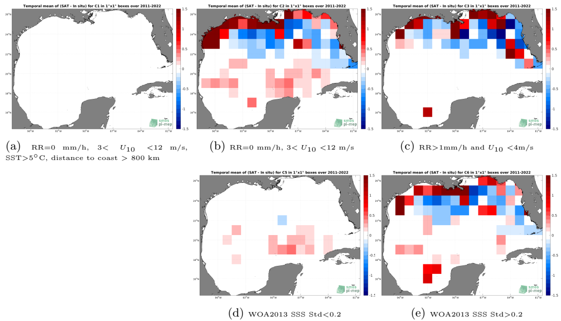
Figure 12: Temporal mean gridded over spatial boxes of size 1^\circ \times 1^\circ of \Delta SSS (SMAP SSS L4 OI v1 - Monthly (IPRC) - TSG (SAMOS)) for 5 different subdatasets corresponding to:RR=0 mm/h, 3 < U_{10} < 12 m/s, SST >5^\circ C, distance to coast > 800 km (a), RR=0 mm/h, 3 < U_{10} < 12 m/s (b), RR >1 mm/h and U_{10} < 4 m/s (c), WOA2013 SSS Std <0.2 (d), WOA2013 SSS Std >0.2 (e).
