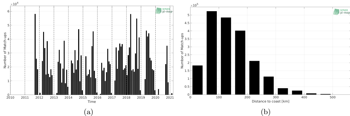
Figure 1: Number of match-ups between TSG (SAMOS) and SMAP SSS L4 OI v1 - Monthly (IPRC) SSS as a function of time (a) and as function of the distance to coast (b) over the Gulf of Mexico Pi-MEP region and for the full satellite product period.
