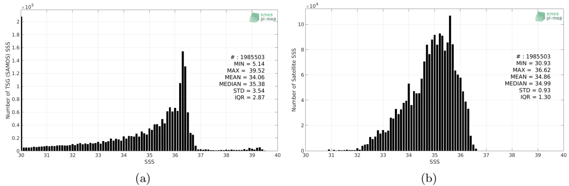
Figure 2: Histograms of SSS from TSG (SAMOS) (a) and SMAP SSS L4 OI v1 - Monthly (IPRC) (b) considering all match-up pairs per bins of 0.1 over the Gulf of Mexico Pi-MEP region and for the full satellite product period.
