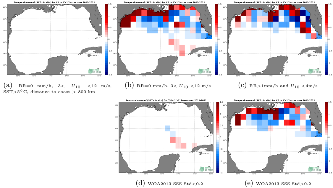
Figure 12: Temporal mean gridded over spatial boxes of size 1^{\circ}\times 1^{\circ} of \Delta\text{SSS} (SMAP SSS L4 OI v1 - Monthly (IPRC) - TSG (SAMOS)) for 5 different subdatasets corresponding to:RR=0 mm/h, 3 < U_{10} < 12 m/s, SST > 5^{\circ}\text{C} , distance to coast > 800 km (a), RR=0 mm/h, 3 < U_{10} < 12 m/s (b), RR > 1 mm/h and U_{10} < 4 m/s (c), WOA2013 SSS Std < 0.2 (d), WOA2013 SSS Std > 0.2 (e).
