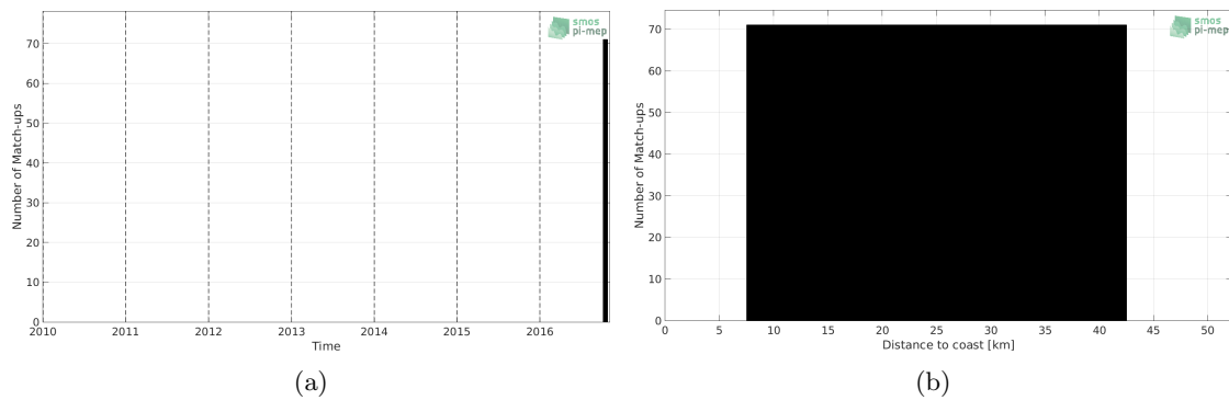
Figure 1: Number of match-ups between TSG (LEGOS-DM) and SMAP SSS L4 OI v1 - Monthly (IPRC) SSS as a function of time (a) and as function of the distance to coast (b) over the Gulf of Mexico Pi-MEP region and for the full satellite product period.
