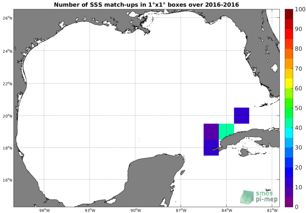
Figure 4: Number of SSS match-ups between TSG (LEGOS-DM) SSS and the SMAP SSS L4 OI v1 - Monthly (IPRC) SSS product for the Gulf of Mexico Pi-MEP region over 1^\circ \times 1^\circ boxes and for the full satellite product period.
