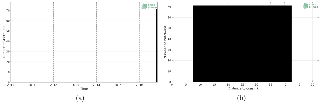
Figure 1: Number of match-ups between TSG (LEGOS-DM) and SMAP SSS L4 OI v1 - Monthly (IPRC) SSS as a function of time (a) and as function of the distance to coast (b) over the Gulf of Mexico Pi-MEP region and for the full satellite product period.
