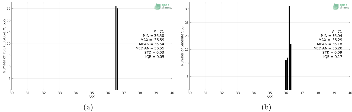
Figure 2: Histograms of SSS from TSG (LEGOS-DM) (a) and SMAP SSS L4 OI v1 - Monthly (IPRC) (b) considering all match-up pairs per bins of 0.1 over the Gulf of Mexico Pi-MEP region and for the full satellite product period.
