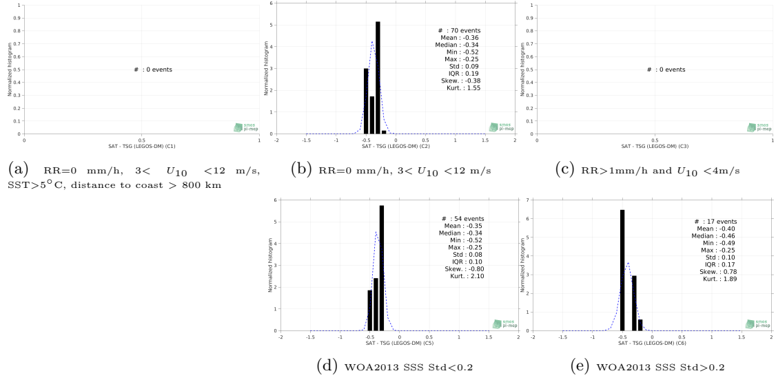
Figure 13: Normalized histogram of \Delta\text{SSS} (SMAP SSS L4 OI v1 - Monthly (IPRC) - TSG (LEGOS-DM)) for 5 different subdatasets corresponding to: RR=0 mm/h, 3 < U_{10} < 12 m/s, SST > 5^{\circ}\text{C} , distance to coast > 800 km (a), RR=0 mm/h, 3 < U_{10} < 12 m/s (b), RR > 1 mm/h and U_{10} < 4 m/s (c), WOA2013 SSS Std < 0.2 (d), WOA2013 SSS Std > 0.2 (e).
