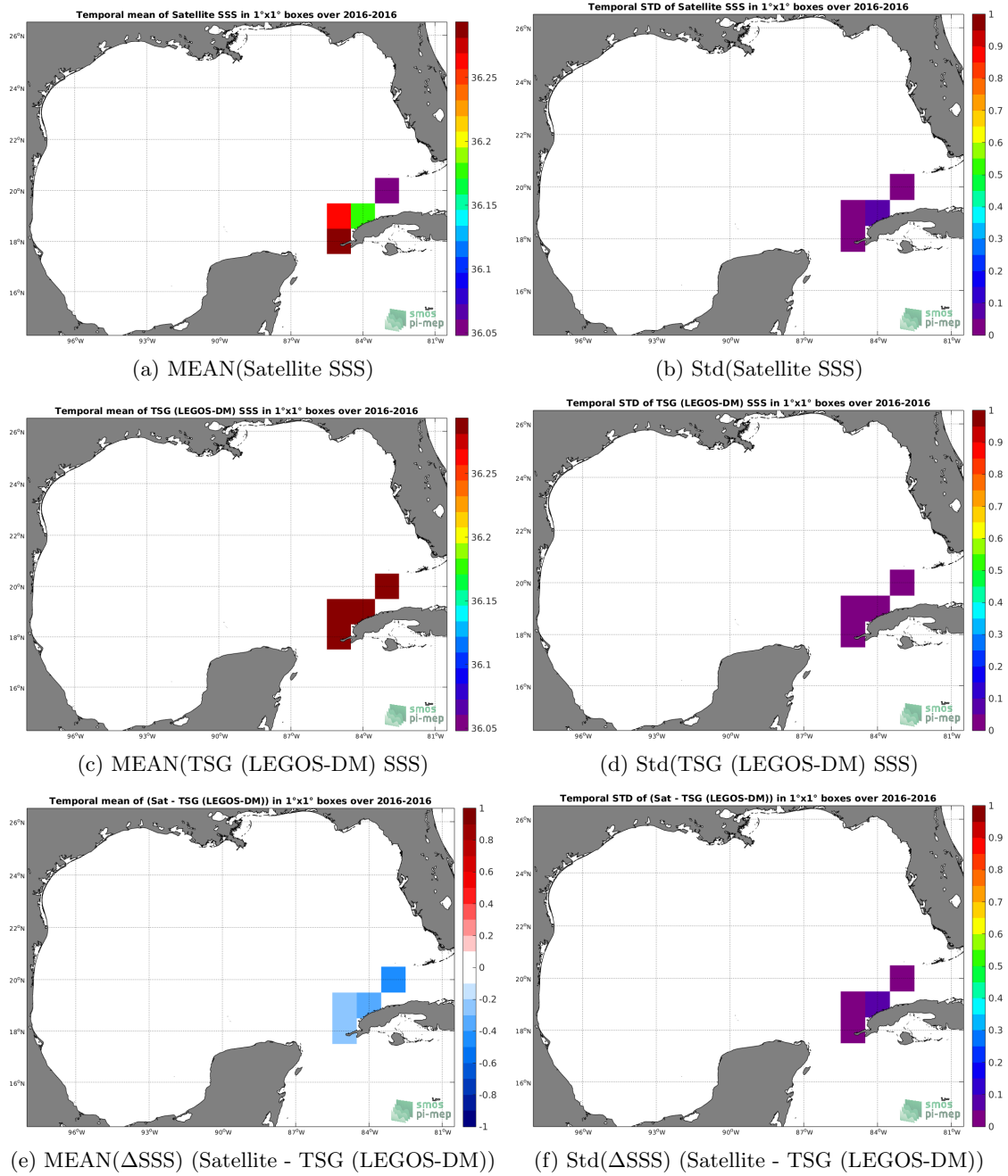
Figure 6: Temporal mean (left) and Std (right) of SSS from SMAP SSS L4 OI v1 - Monthly (IPRC) (top), TSG (LEGOS-DM) (middle), and of \Delta SSS (Satellite - TSG (LEGOS-DM)). Only match-up pairs are used to generate these maps.
