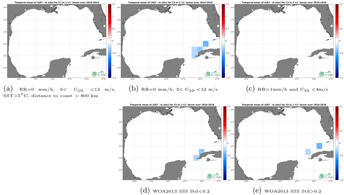
Figure 12: Temporal mean gridded over spatial boxes of size 1^{\circ}\times 1^{\circ} of \Delta\text{SSS} (SMAP SSS L4 OI v1 - Monthly (IPRC) - TSG (LEGOS-DM)) for 5 different subdatasets corresponding to:RR=0 mm/h, 3 < U_{10} < 12 m/s, SST >5^{\circ}\text{C} , distance to coast > 800 km (a), RR=0 mm/h, 3 < U_{10} < 12 m/s (b), RR >1 mm/h and U_{10} < 4 m/s (c), WOA2013 SSS Std <0.2 (d), WOA2013 SSS Std >0.2 (e).
