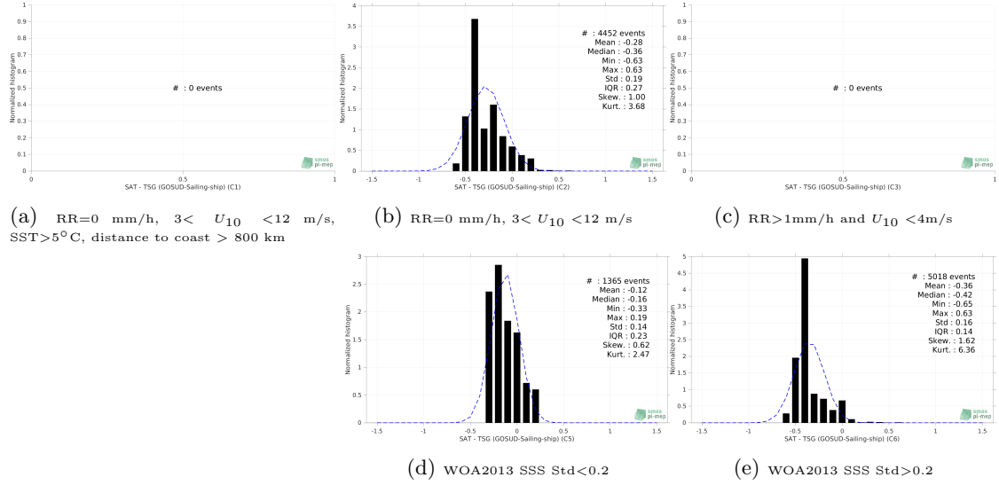
Figure 13: Normalized histogram of \Delta SSS (SMAP SSS L4 OI v1 - Monthly (IPRC) - TSG (GOSUD-Sailing-ship)) for 5 different subdatasets corresponding to: RR=0 mm/h, 3 < U_{10} < 12 m/s, SST > 5°C, distance to coast > 800 km (a), RR=0 mm/h, 3 < U_{10} < 12 m/s (b), RR > 1mm/h and U_{10} < 4 m/s (c), WOA2013 SSS Std < 0.2 (d), WOA2013 SSS Std > 0.2 (e).
