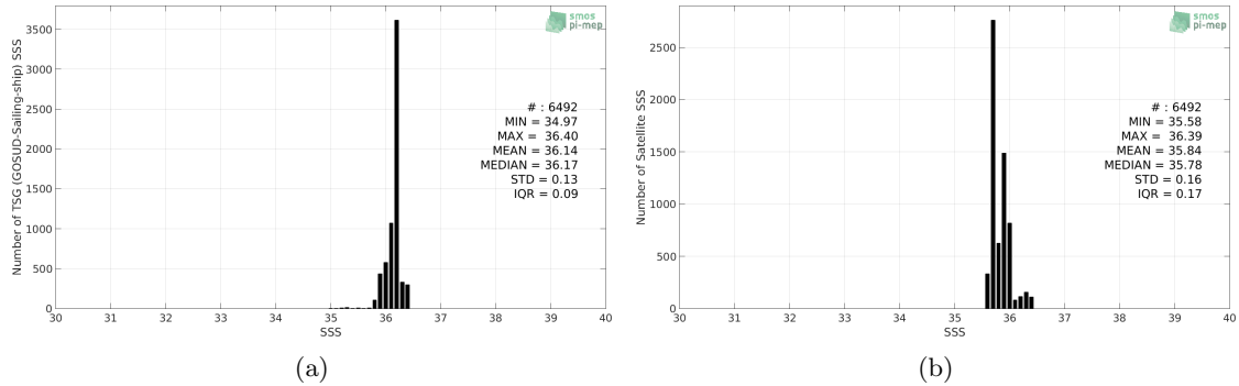
Figure 2: Histograms of SSS from TSG (GOSUD-Sailing-ship) (a) and SMAP SSS L4 OI v1 - Monthly (IPRC) (b) considering all match-up pairs per bins of 0.1 over the Gulf of Mexico Pi-MEP region and for the full satellite product period.
