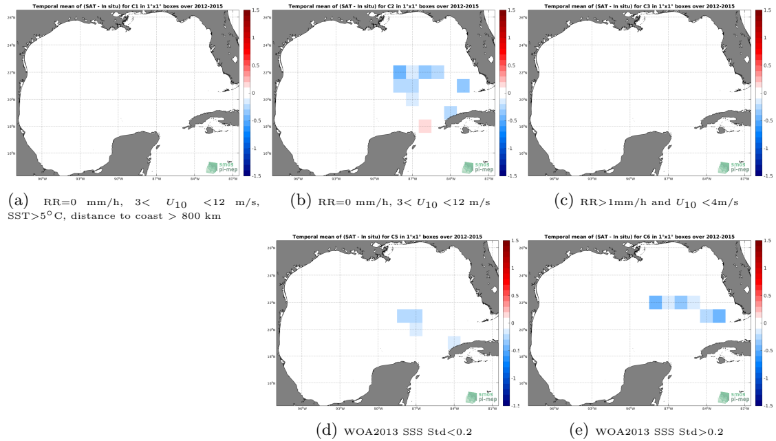
Figure 12: Temporal mean gridded over spatial boxes of size 1^\circ \times 1^\circ of \Delta SSS (SMAP SSS L4 OI v1 - Monthly (IPRC) - TSG (GOSUD-Sailing-ship)) for 5 different subdatasets corresponding to: RR=0 mm/h, 3 < U_{10} < 12 m/s, SST >5^\circ\text{C} , distance to coast > 800 km (a), RR=0 mm/h, 3 < U_{10} < 12 m/s (b), RR >1 mm/h and U_{10} < 4 m/s (c), WOA2013 SSS Std <0.2 (d), WOA2013 SSS Std >0.2 (e).
