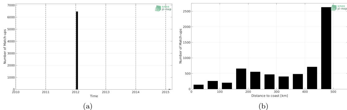
Figure 1: Number of match-ups between TSG (GOSUD-Sailing-ship) and SMAP SSS L4 OI v1 - Monthly (IPRC) SSS as a function of time (a) and as function of the distance to coast (b) over the Gulf of Mexico Pi-MEP region and for the full satellite product period.
