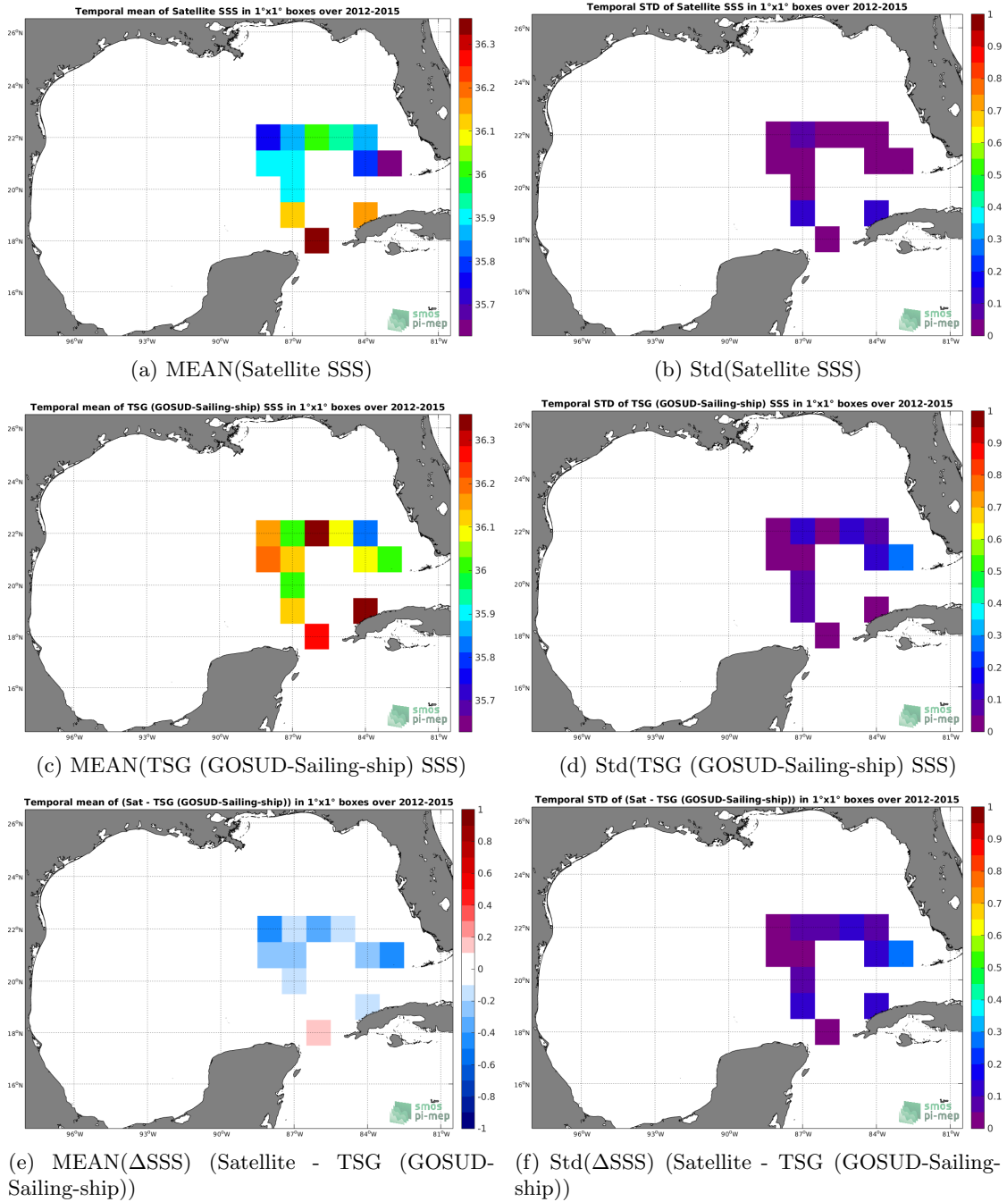
Figure 6: Temporal mean (left) and Std (right) of SSS from SMAP SSS L4 OI v1 - Monthly (IPRC) (top), TSG (GOSUD-Sailing-ship) (middle), and of \Delta SSS (Satellite - TSG (GOSUD-Sailing-ship)). Only match-up pairs are used to generate these maps.
