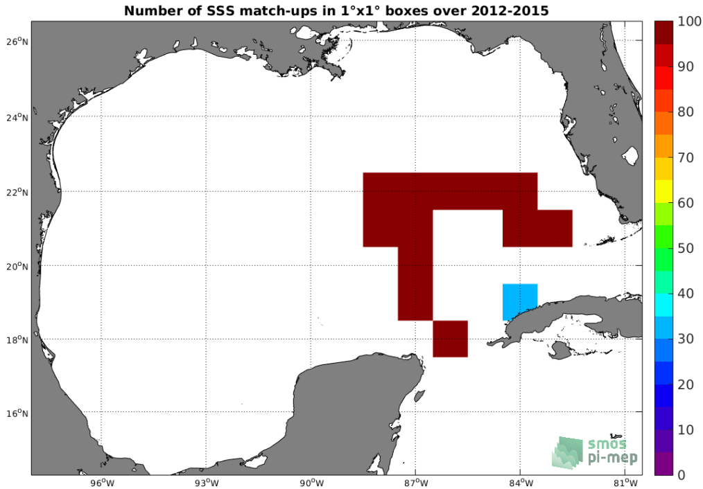
Figure 4: Number of SSS match-ups between TSG (GOSUD-Sailing-ship) SSS and the SMAP SSS L4 OI v1 - Monthly (IPRC) SSS product for the Gulf of Mexico Pi-MEP region over 1°x1° boxes and for the full satellite product period.
