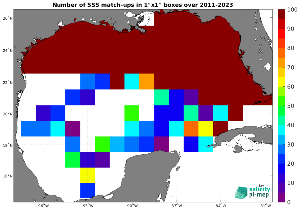
Figure 5: Number of SSS match-ups between TSG (SAMOS) SSS and the SMAP SSS L4 OI v3 - Monthly (ESR) SSS product for the Gulf of Mexico Pi-MEP region over 1^\circ \times 1^\circ boxes and for the full satellite product period.
