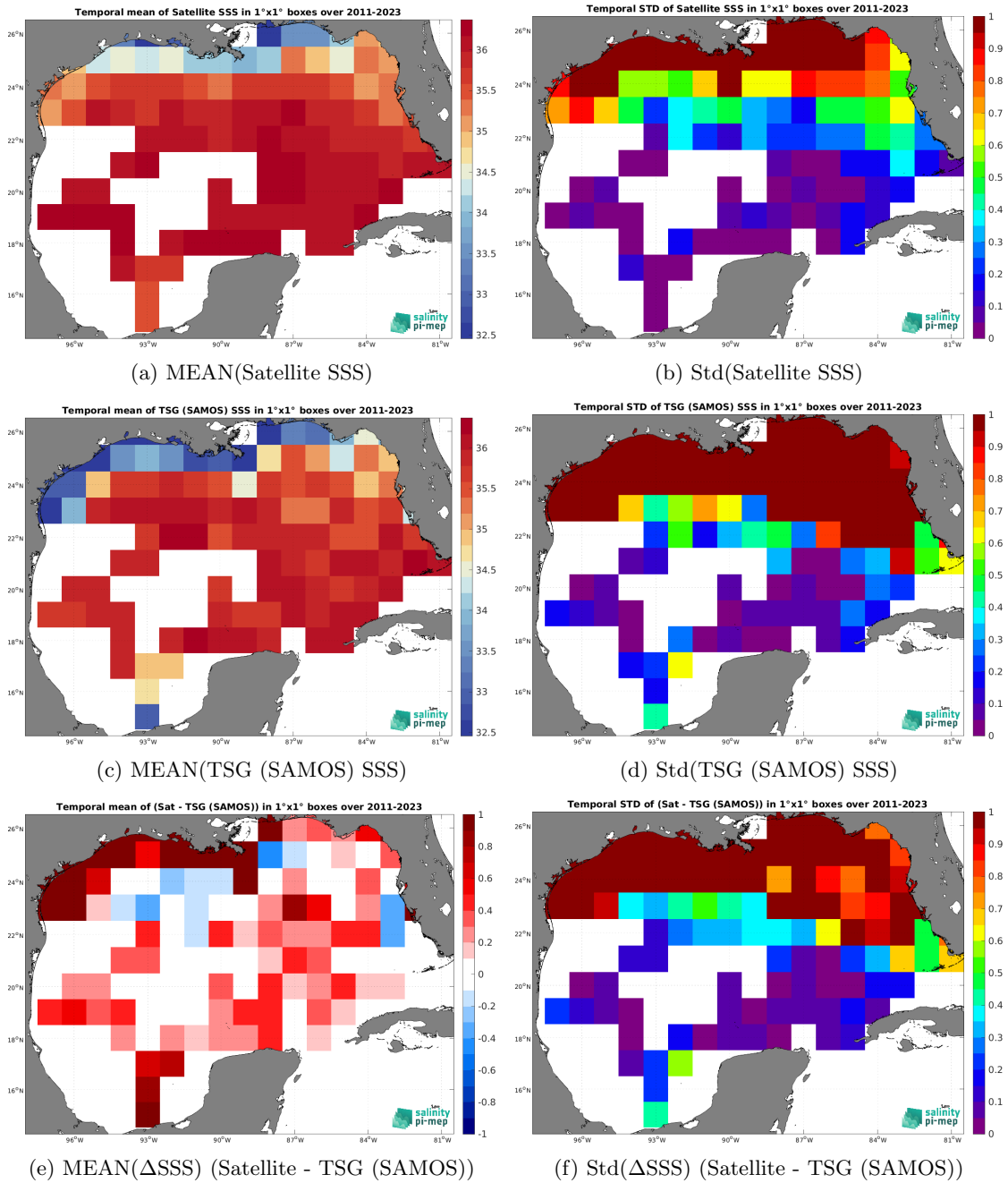
Figure 7: Temporal mean (left) and Std (right) of SSS from SMAP SSS L4 OI v3 - Monthly (ESR) (top), TSG (SAMOS) (middle), and of \Delta SSS (Satellite - TSG (SAMOS)). Only match-up pairs are used to generate these maps.
