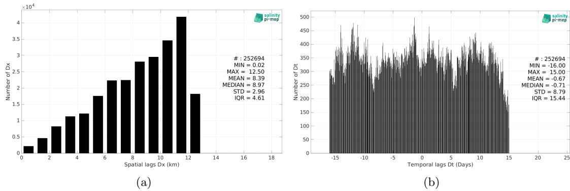
Figure 6: Histograms of the spatial (a) and temporal (b) lags between the location/time of the TSG (SAMOS) measurement and the date of the corresponding SMAP SSS L4 OI v3 - Monthly (ESR) SSS pixel.
