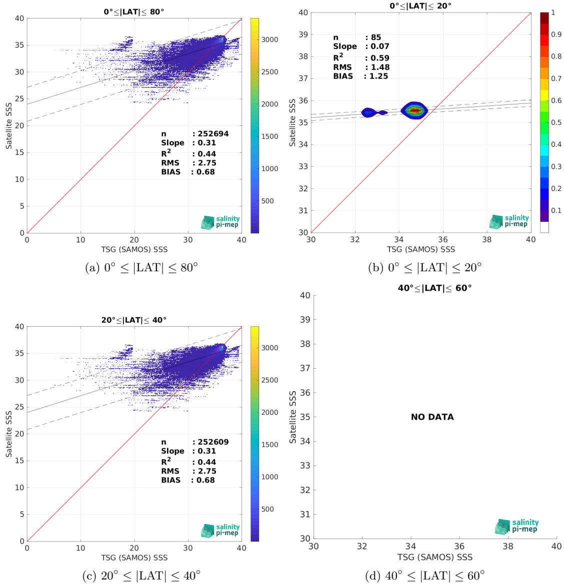
Figure 10: Contour maps of the concentration of SMAP SSS L4 OI v3 - Monthly (ESR) SSS (y-axis) versus TSG (SAMOS) SSS (x-axis) at match-up pairs for different latitude bands. For each plot, the red line shows x=y . The black thin and dashed lines indicate a linear fit through the data cloud and the \pm 95\% confidence levels, respectively. The number match-up pairs n , the slope and R^2 coefficient of the linear fit, the root mean square (RMS) and the mean bias between satellite and in situ data are indicated for each latitude band in each plots.
