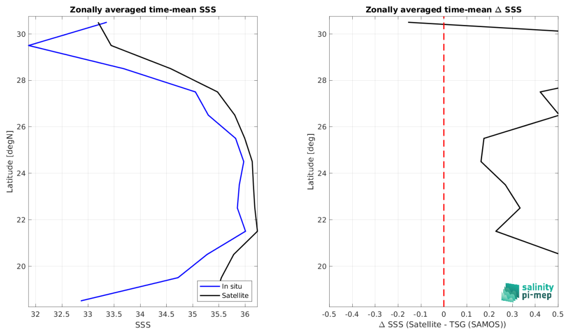
Figure 9: Left panel: Zonal mean SSS from SMAP SSS L4 OI v3 - Monthly (ESR) satellite product (black) and from TSG (SAMOS) (blue). Right panel: Zonal mean of \Delta SSS (Satellite - TSG (SAMOS)) for all the collected Pi-MEP match-up pairs estimated over the full satellite product period.
