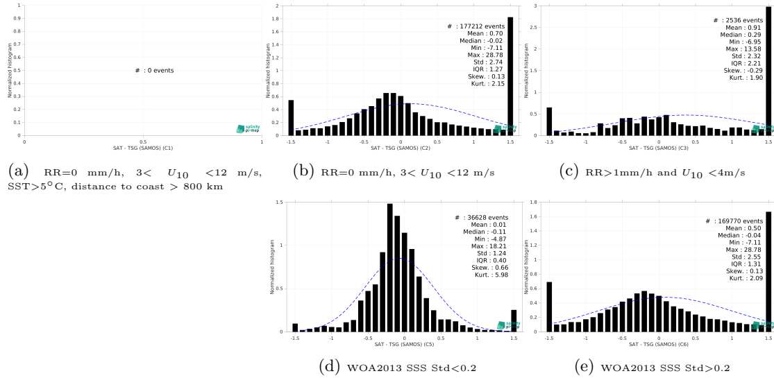
Figure 15: Normalized histogram of \Delta SSS (SMAP SSS L4 OI v3 - Monthly (ESR) - TSG (SAMOS)) for 5 different subdatasets corresponding to: RR=0 mm/h, 3 < U_{10} < 12 m/s, SST > 5°C, distance to coast > 800 km (a), RR=0 mm/h, 3 < U_{10} < 12 m/s (b), RR > 1mm/h and U_{10} < 4 m/s (c), WOA2013 SSS Std < 0.2 (d), WOA2013 SSS Std > 0.2 (e).
