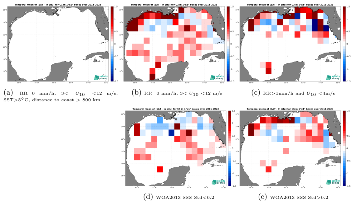
Figure 14: Temporal mean gridded over spatial boxes of size 1^\circ \times 1^\circ of \Delta SSS (SMAP SSS L4 OI v3 - Monthly (ESR) - TSG (SAMOS)) for 5 different subdatasets corresponding to:RR=0 mm/h, 3 < U_{10} < 12 m/s, SST >5^\circ\text{C} , distance to coast > 800 km (a), RR=0 mm/h, 3 < U_{10} < 12 m/s (b), RR >1 mm/h and U_{10} < 4 m/s (c), WOA2013 SSS Std <0.2 (d), WOA2013 SSS Std >0.2 (e).
