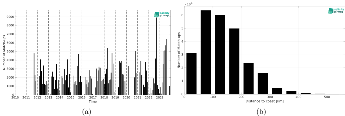
Figure 2: Number of match-ups between TSG (SAMOS) and SMAP SSS L4 OI v3 - Monthly (ESR) SSS as a function of time (a) and as function of the distance to coast (b) over the Gulf of Mexico Pi-MEP region and for the full satellite product period.
