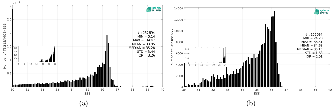
Figure 3: Histograms of SSS from TSG (SAMOS) (a) and SMAP SSS L4 OI v3 - Monthly (ESR) (b) considering all match-up pairs per bins of 0.1 over the Gulf of Mexico Pi-MEP region and for the full satellite product period.
