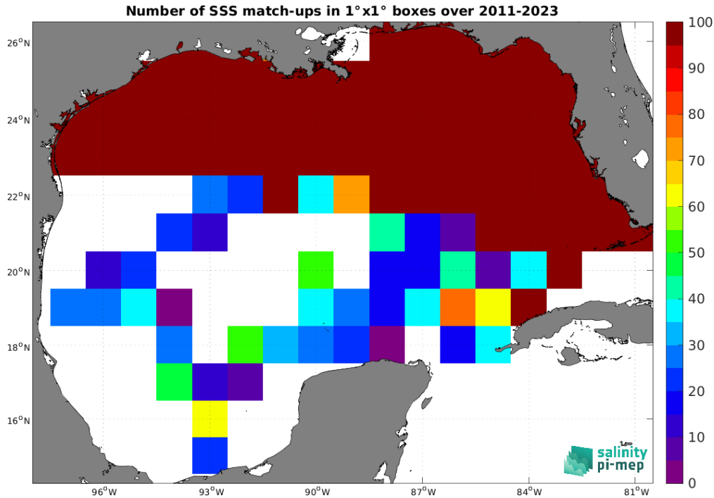
Figure 5: Number of SSS match-ups between TSG (SAMOS) SSS and the SMAP SSS L4 OI v3 - Monthly (ESR) SSS product for the Gulf of Mexico Pi-MEP region over 1°×1° boxes and for the full satellite product period.
