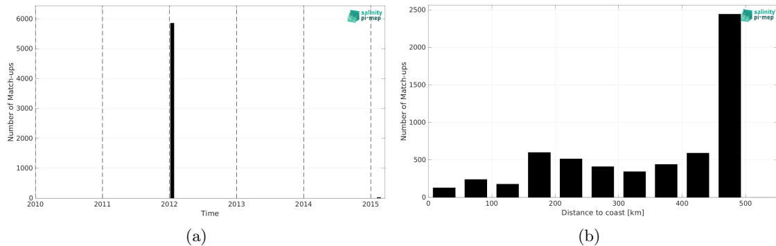
Figure 2: Number of match-ups between TSG (GOSUD-Sailing-ship) and SMAP SSS L4 OI v3 - Monthly (ESR) SSS as a function of time (a) and as function of the distance to coast (b) over the Gulf of Mexico Pi-MEP region and for the full satellite product period.
