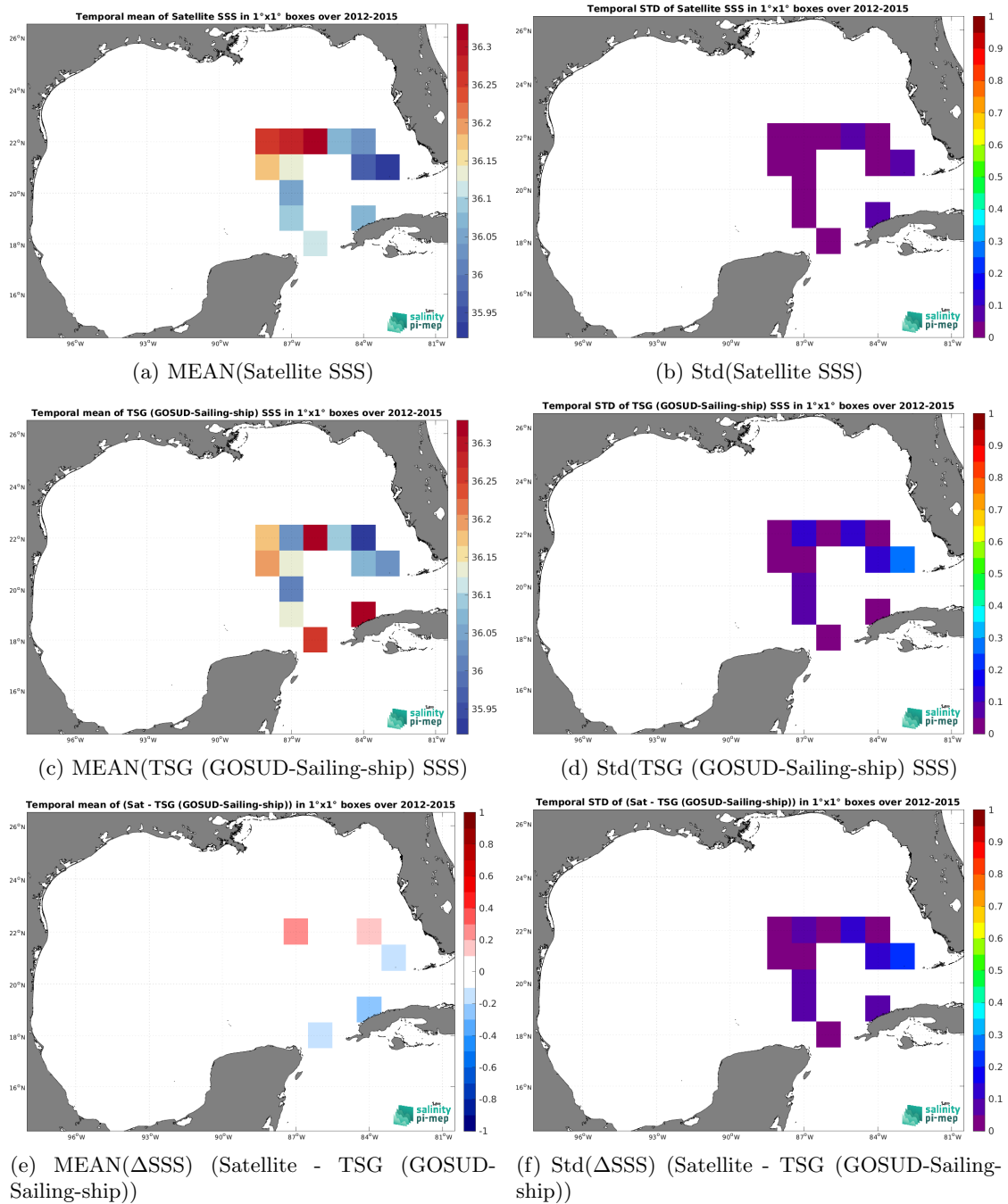
Figure 7: Temporal mean (left) and Std (right) of SSS from SMAP SSS L4 OI v3 - Monthly (ESR) (top), TSG (GOSUD-Sailing-ship) (middle), and of \Delta SSS (Satellite - TSG (GOSUD-Sailing-ship)). Only match-up pairs are used to generate these maps.
