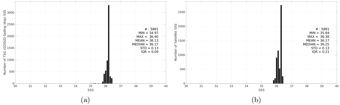
Figure 3: Histograms of SSS from TSG (GOSUD-Sailing-ship) (a) and SMAP SSS L4 OI v3 - Monthly (ESR) (b) considering all match-up pairs per bins of 0.1 over the Gulf of Mexico Pi-MEP region and for the full satellite product period.
