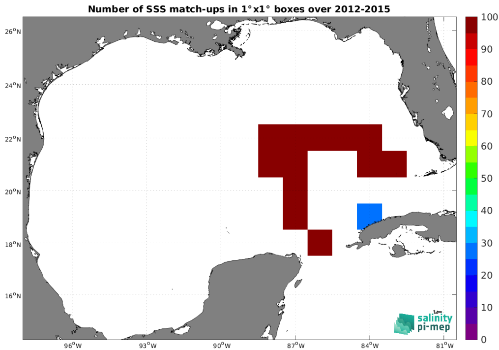
Figure 5: Number of SSS match-ups between TSG (GOSUD-Sailing-ship) SSS and the SMAP SSS L4 OI v3 - Monthly (ESR) SSS product for the Gulf of Mexico Pi-MEP region over 1°x1° boxes and for the full satellite product period.
