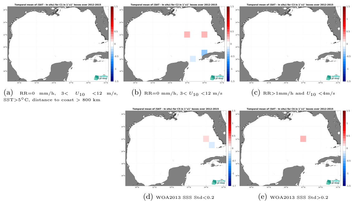
Figure 14: Temporal mean gridded over spatial boxes of size 1^\circ \times 1^\circ of \Delta\text{SSS} (SMAP SSS L4 OI v3 - Monthly (ESR) - TSG (GOSUD-Sailing-ship)) for 5 different subdatasets corresponding to:RR=0 mm/h, 3 < U_{10} < 12 m/s, SST>5°C, distance to coast > 800 km (a), RR=0 mm/h, 3 < U_{10} < 12 m/s (b), RR>1mm/h and U_{10} < 4 m/s (c), WOA2013 SSS Std<0.2 (d), WOA2013 SSS Std>0.2 (e).
