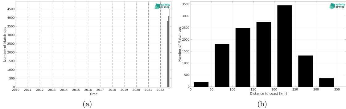
Figure 2: Number of match-ups between Saildrone and SMAP SSS L4 OI v3 - Monthly (ESR) SSS as a function of time (a) and as function of the distance to coast (b) over the Gulf of Mexico Pi-MEP region and for the full satellite product period.
