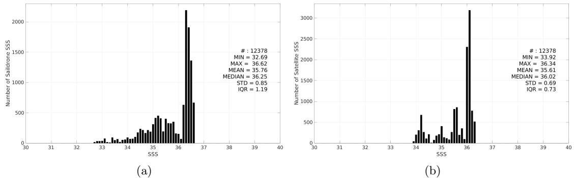
Figure 3: Histograms of SSS from Saildrone (a) and SMAP SSS L4 OI v3 - Monthly (ESR) (b) considering all match-up pairs per bins of 0.1 over the Gulf of Mexico Pi-MEP region and for the full satellite product period.
