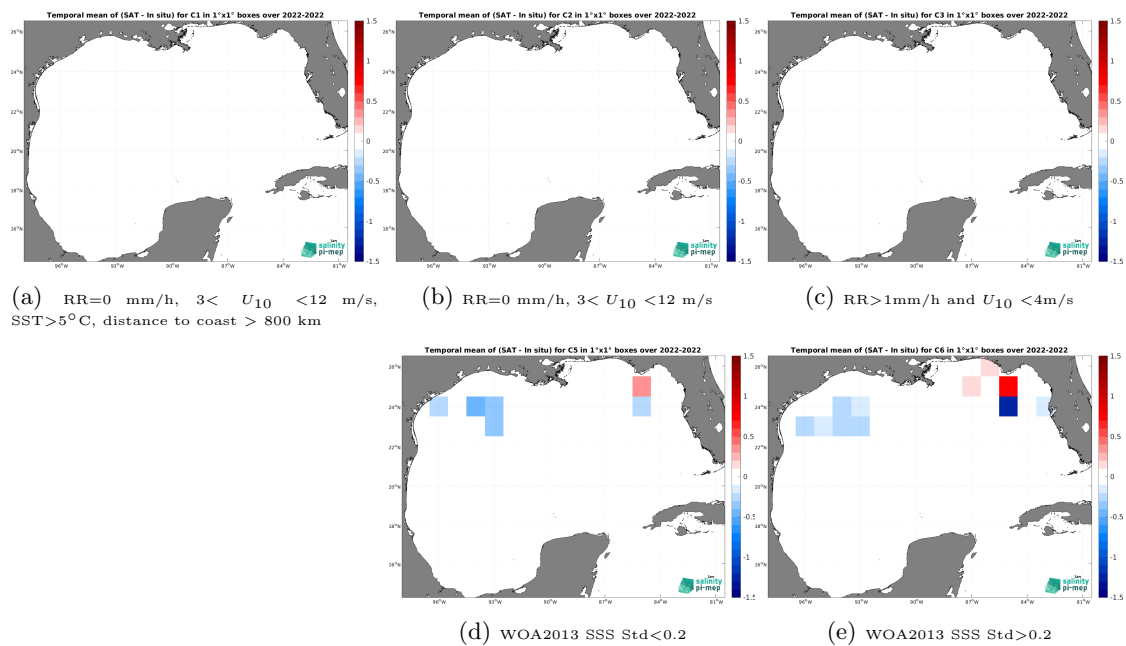
Figure 14: Temporal mean gridded over spatial boxes of size 1^\circ \times 1^\circ of \Delta SSS (SMAP SSS L4 OI v3 - Monthly (ESR) - Saildrone) for 5 different subdatasets corresponding to:RR=0 mm/h, 3 < U_{10} < 12 m/s, SST >5^\circ C, distance to coast > 800 km (a), RR=0 mm/h, 3 < U_{10} < 12 m/s (b), RR >1 mm/h and U_{10} < 4 m/s (c), WOA2013 SSS Std <0.2 (d), WOA2013 SSS Std >0.2 (e).
