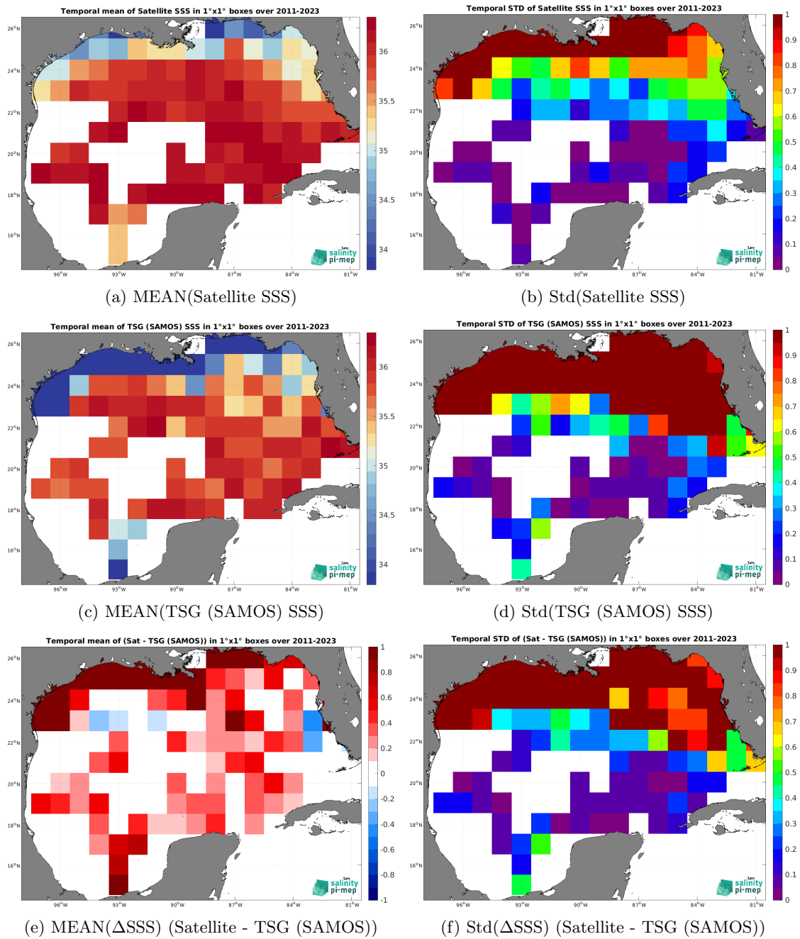
Figure 7: Temporal mean (left) and Std (right) of SSS from SMAP SSS L4 OI v3 - Daily (ESR) (top), TSG (SAMOS) (middle), and of \Delta SSS (Satellite - TSG (SAMOS)). Only match-up pairs are used to generate these maps.
