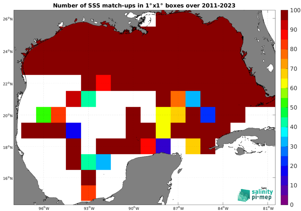
Figure 5: Number of SSS match-ups between TSG (SAMOS) SSS and the SMAP SSS L4 OI v3 - Daily (ESR) SSS product for the Gulf of Mexico Pi-MEP region over 1^\circ \times 1^\circ boxes and for the full satellite product period.
