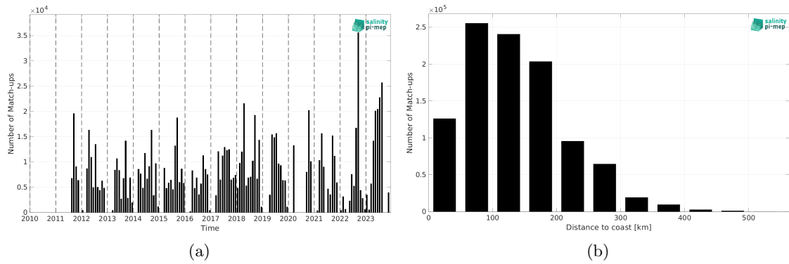
Figure 2: Number of match-ups between TSG (SAMOS) and SMAP SSS L4 OI v3 - Daily (ESR) SSS as a function of time (a) and as function of the distance to coast (b) over the Gulf of Mexico Pi-MEP region and for the full satellite product period.
