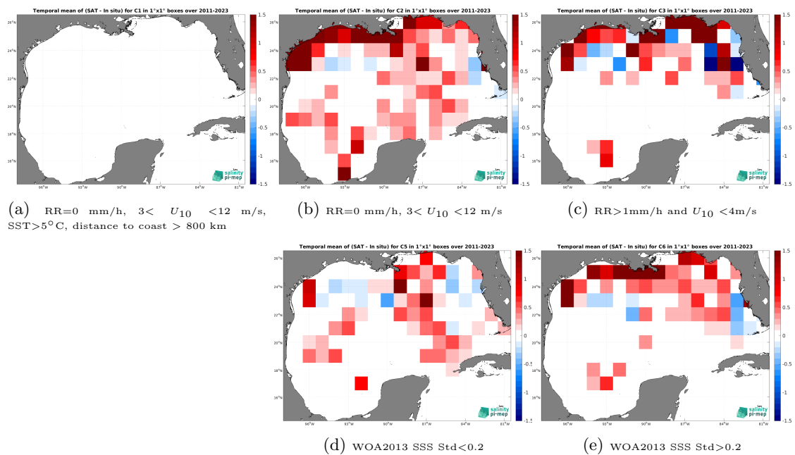
Figure 14: Temporal mean gridded over spatial boxes of size 1^\circ \times 1^\circ of \Delta SSS (SMAP SSS L4 OI v3 - Daily (ESR) - TSG (SAMOS)) for 5 different subdatasets corresponding to:RR=0 mm/h, 3 < U_{10} < 12 m/s, SST >5^\circ C, distance to coast > 800 km (a), RR=0 mm/h, 3 < U_{10} < 12 m/s (b), RR >1 mm/h and U_{10} < 4 m/s (c), WOA2013 SSS Std <0.2 (d), WOA2013 SSS Std >0.2 (e).
