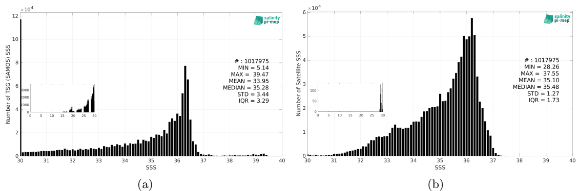
Figure 3: Histograms of SSS from TSG (SAMOS) (a) and SMAP SSS L4 OI v3 - Daily (ESR) (b) considering all match-up pairs per bins of 0.1 over the Gulf of Mexico Pi-MEP region and for the full satellite product period.
