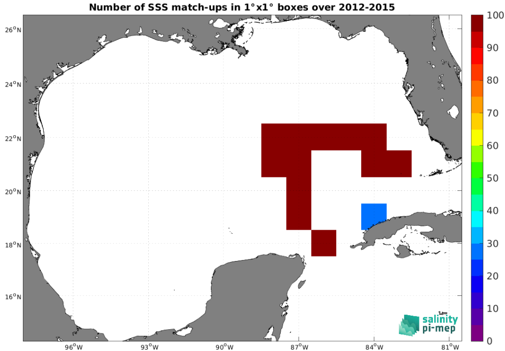
Figure 5: Number of SSS match-ups between TSG (GOSUD-Sailing-ship) SSS and the SMAP SSS L4 OI v3 - Daily (ESR) SSS product for the Gulf of Mexico Pi-MEP region over 1^\circ \times 1^\circ boxes and for the full satellite product period.
