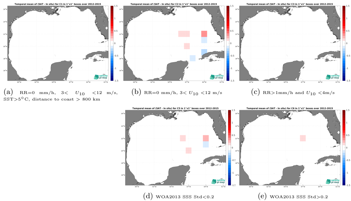
Figure 14: Temporal mean gridded over spatial boxes of size 1^\circ \times 1^\circ of \Delta\text{SSS} (SMAP SSS L4 OI v3 - Daily (ESR) - TSG (GOSUD-Sailing-ship)) for 5 different subdatasets corresponding to:RR=0 mm/h, 3 < U_{10} < 12 m/s, SST>5°C, distance to coast > 800 km (a), RR=0 mm/h, 3 < U_{10} < 12 m/s (b), RR>1mm/h and U_{10} < 4 m/s (c), WOA2013 SSS Std<0.2 (d), WOA2013 SSS Std>0.2 (e).
