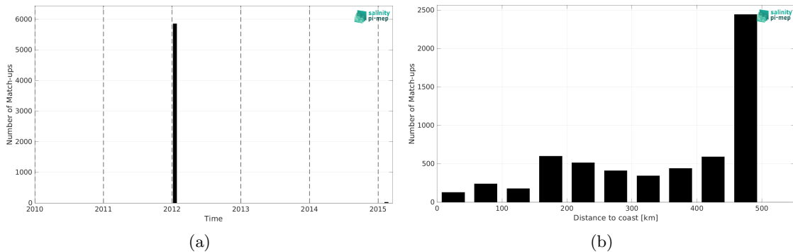
Figure 2: Number of match-ups between TSG (GOSUD-Sailing-ship) and SMAP SSS L4 OI v3 - Daily (ESR) SSS as a function of time (a) and as function of the distance to coast (b) over the Gulf of Mexico Pi-MEP region and for the full satellite product period.
