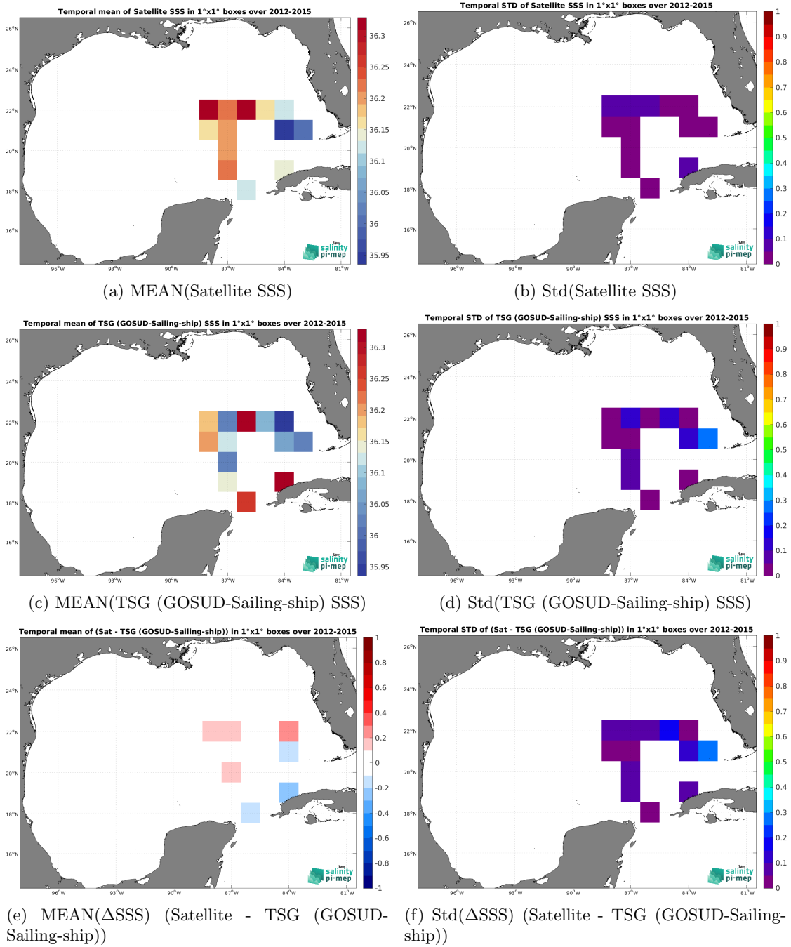
Figure 7: Temporal mean (left) and Std (right) of SSS from SMAP SSS L4 OI v3 - Daily (ESR) (top), TSG (GOSUD-Sailing-ship) (middle), and of \Delta SSS (Satellite - TSG (GOSUD-Sailing-ship)). Only match-up pairs are used to generate these maps.
