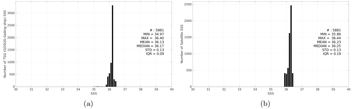
Figure 3: Histograms of SSS from TSG (GOSUD-Sailing-ship) (a) and SMAP SSS L4 OI v3 - Daily (ESR) (b) considering all match-up pairs per bins of 0.1 over the Gulf of Mexico Pi-MEP region and for the full satellite product period.
