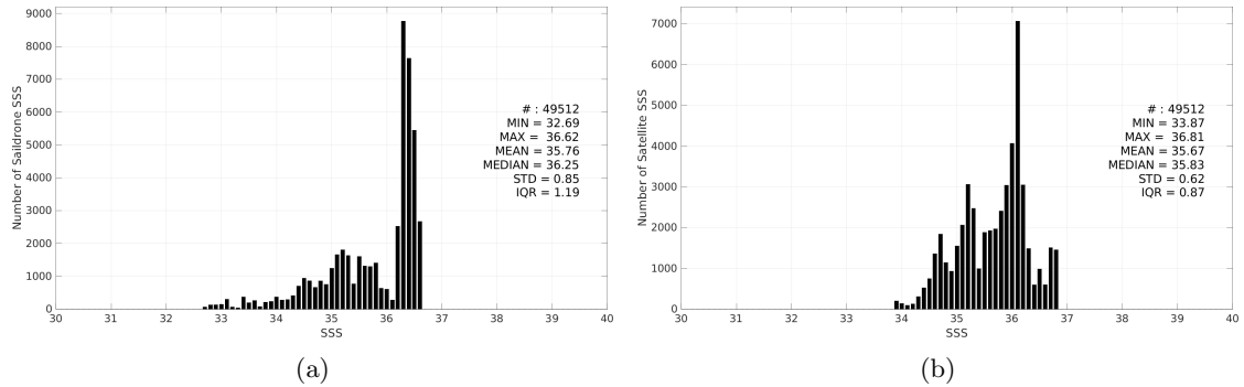
Figure 3: Histograms of SSS from Saildrone (a) and SMAP SSS L4 OI v3 - Daily (ESR) (b) considering all match-up pairs per bins of 0.1 over the Gulf of Mexico Pi-MEP region and for the full satellite product period.
