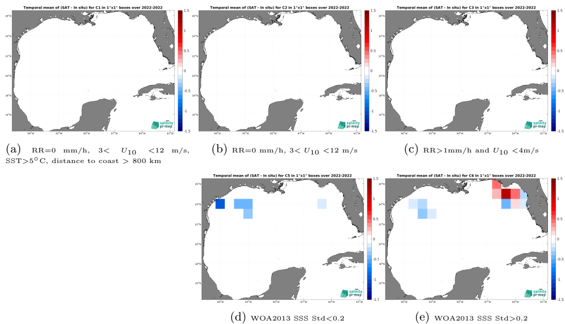
Figure 14: Temporal mean gridded over spatial boxes of size 1^\circ \times 1^\circ of \Delta SSS (SMAP SSS L4 OI v3 - Daily (ESR) - Saildrone) for 5 different subdatasets corresponding to:RR=0 mm/h, 3 < U_{10} < 12 m/s, SST >5^\circ C, distance to coast > 800 km (a), RR=0 mm/h, 3 < U_{10} < 12 m/s (b), RR >1 mm/h and U_{10} < 4 m/s (c), WOA2013 SSS Std <0.2 (d), WOA2013 SSS Std >0.2 (e).
