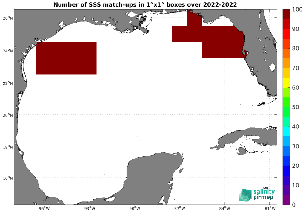
Figure 5: Number of SSS match-ups between Saildrone SSS and the SMAP SSS L4 OI v3 - Daily (ESR) SSS product for the Gulf of Mexico Pi-MEP region over 1^\circ \times 1^\circ boxes and for the full satellite product period.
