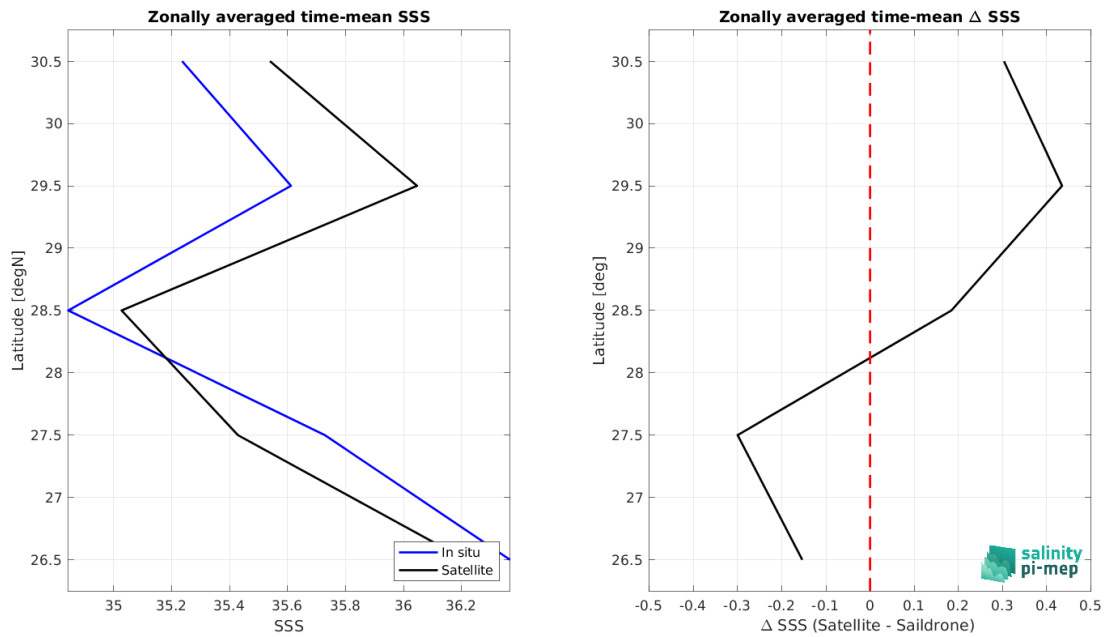
Figure 9: Left panel: Zonal mean SSS from SMAP SSS L4 OI v3 - Daily (ESR) satellite product (black) and from Sairdron (blue). Right panel: Zonal mean of \Delta SSS (Satellite - Sairdron) for all the collected Pi-MEP match-up pairs estimated over the full satellite product period.
