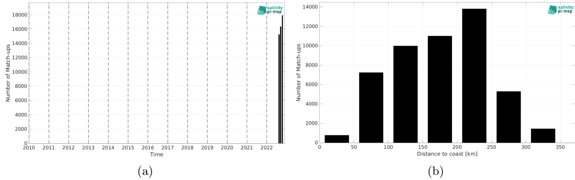
Figure 2: Number of match-ups between Saildrone and SMAP SSS L4 OI v3 - Daily (ESR) SSS as a function of time (a) and as function of the distance to coast (b) over the Gulf of Mexico Pi-MEP region and for the full satellite product period.
