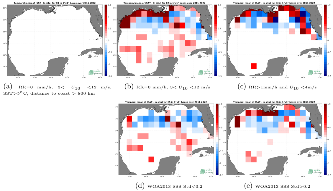
Figure 12: Temporal mean gridded over spatial boxes of size 1^\circ \times 1^\circ of \Delta SSS (SMAP SSS L4 OI v2 - 7 Days (ESR) - TSG (SAMOS)) for 5 different subdatasets corresponding to:RR=0 mm/h, 3 < U_{10} < 12 m/s, SST >5^\circ C, distance to coast > 800 km (a), RR=0 mm/h, 3 < U_{10} < 12 m/s (b), RR >1 mm/h and U_{10} < 4 m/s (c), WOA2013 SSS Std <0.2 (d), WOA2013 SSS Std >0.2 (e).
