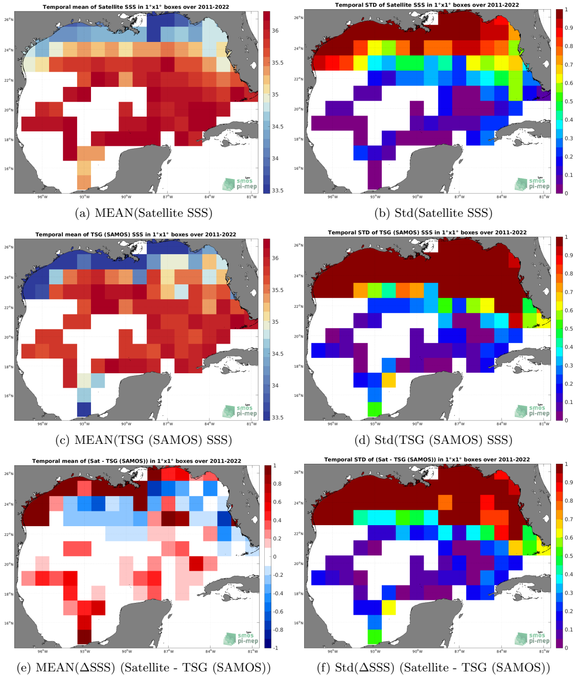
Figure 6: Temporal mean (left) and Std (right) of SSS from SMAP SSS L4 OI v2 - 7 Days (ESR) (top), TSG (SAMOS) (middle), and of \Delta SSS (Satellite - TSG (SAMOS)). Only match-up pairs are used to generate these maps.
