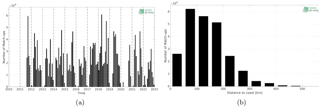
Figure 1: Number of match-ups between TSG (SAMOS) and SMAP SSS L4 OI v2 - 7 Days (ESR) SSS as a function of time (a) and as function of the distance to coast (b) over the Gulf of Mexico Pi-MEP region and for the full satellite product period.
