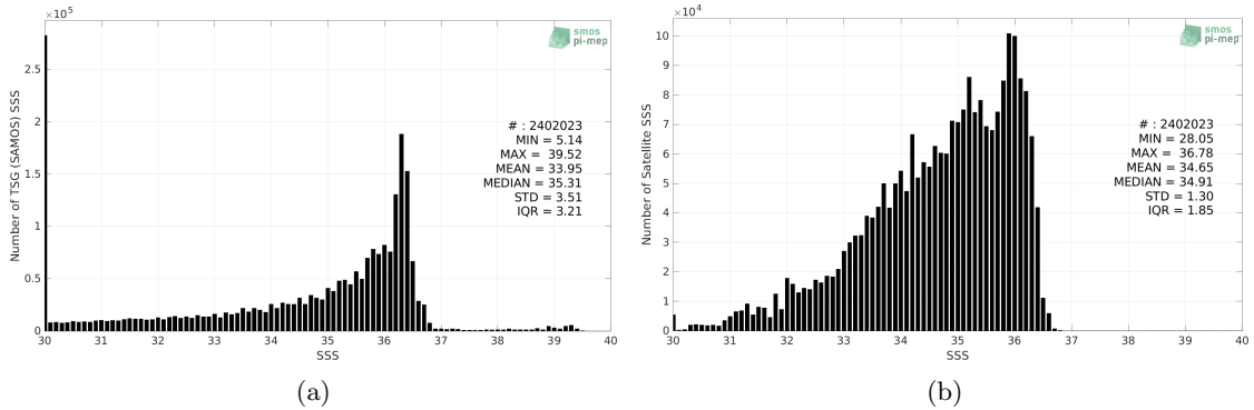
Figure 2: Histograms of SSS from TSG (SAMOS) (a) and SMAP SSS L4 OI v2 - 7 Days (ESR) (b) considering all match-up pairs per bins of 0.1 over the Gulf of Mexico Pi-MEP region and for the full satellite product period.
