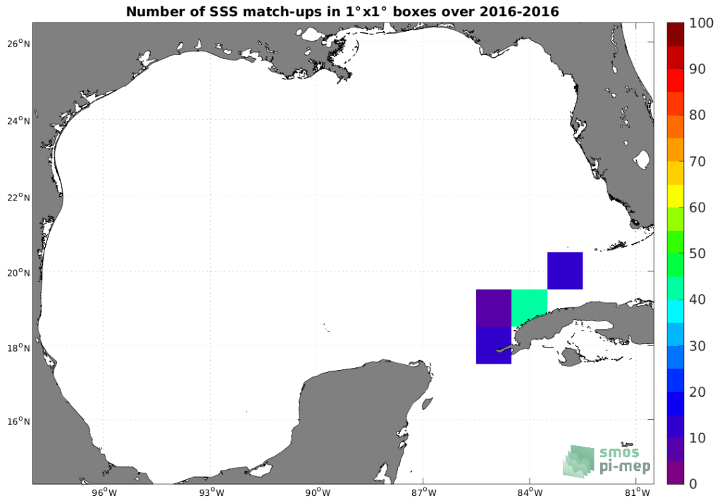
Figure 4: Number of SSS match-ups between TSG (LEGOS-DM) SSS and the SMAP SSS L4 OI v2 - 7 Days (ESR) SSS product for the Gulf of Mexico Pi-MEP region over 1^\circ \times 1^\circ boxes and for the full satellite product period.
