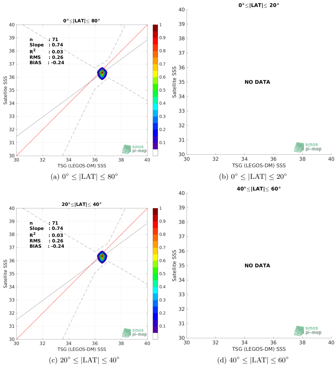
Figure 9: Contour maps of the concentration of SMAP SSS L4 OI v2 - 7 Days (ESR) SSS (y-axis) versus TSG (LEGOS-DM) SSS (x-axis) at match-up pairs for different latitude bands. For each plot, the red line shows x=y . The black thin and dashed lines indicate a linear fit through the data cloud and the \pm 95\% confidence levels, respectively. The number match-up pairs n , the slope and R^2 coefficient of the linear fit, the root mean square (RMS) and the mean bias between satellite and in situ data are indicated for each latitude band in each plots.
