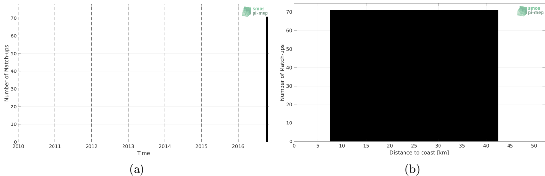
Figure 1: Number of match-ups between TSG (LEGOS-DM) and SMAP SSS L4 OI v2 - 7 Days (ESR) SSS as a function of time (a) and as function of the distance to coast (b) over the Gulf of Mexico Pi-MEP region and for the full satellite product period.
