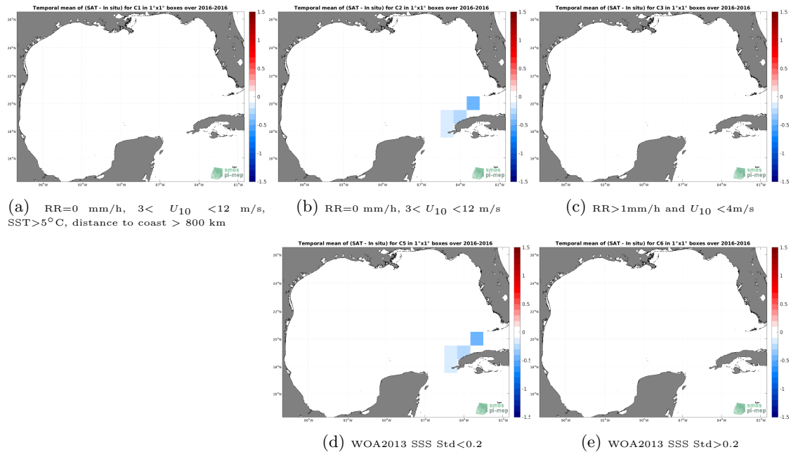
Figure 12: Temporal mean gridded over spatial boxes of size 1^{\circ}\times 1^{\circ} of \Delta\text{SSS} (SMAP SSS L4 OI v2 - 7 Days (ESR) - TSG (LEGOS-DM)) for 5 different subdatasets corresponding to:RR=0 mm/h, 3 < U_{10} < 12 m/s, SST >5^{\circ}\text{C} , distance to coast > 800 km (a), RR=0 mm/h, 3 < U_{10} < 12 m/s (b), RR >1 mm/h and U_{10} < 4 m/s (c), WOA2013 SSS Std <0.2 (d), WOA2013 SSS Std >0.2 (e).
