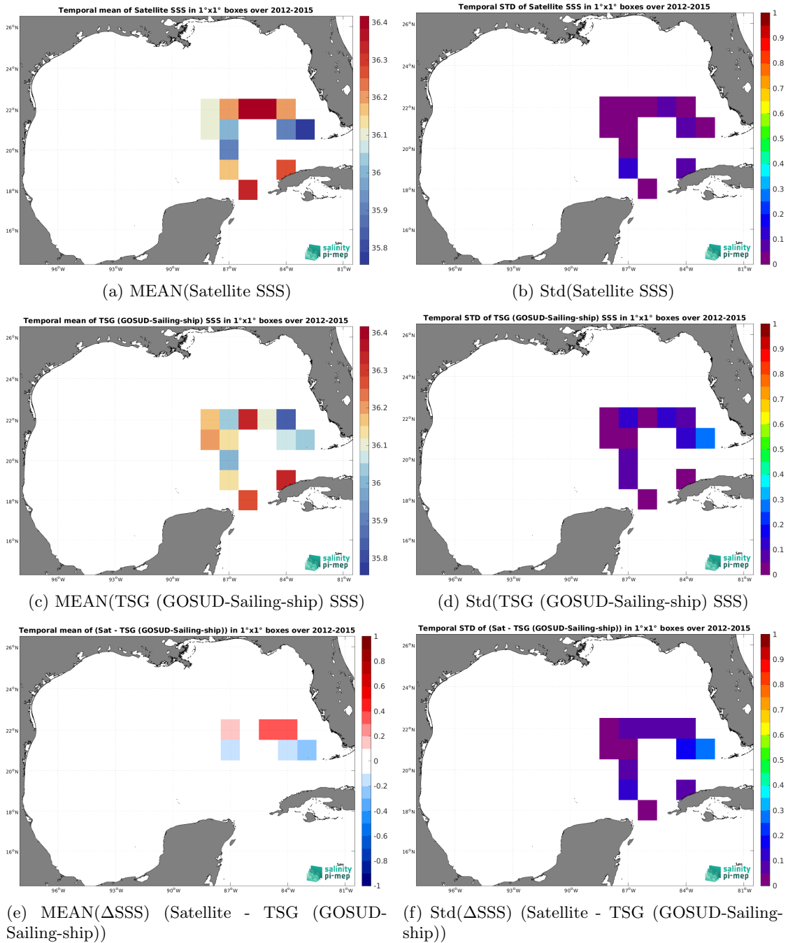
Figure 6: Temporal mean (left) and Std (right) of SSS from SMAP SSS L4 OI v2 - 7 Days (ESR) (top), TSG (GOSUD-Sailing-ship) (middle), and of \Delta SSS (Satellite - TSG (GOSUD-Sailing-ship)). Only match-up pairs are used to generate these maps.
