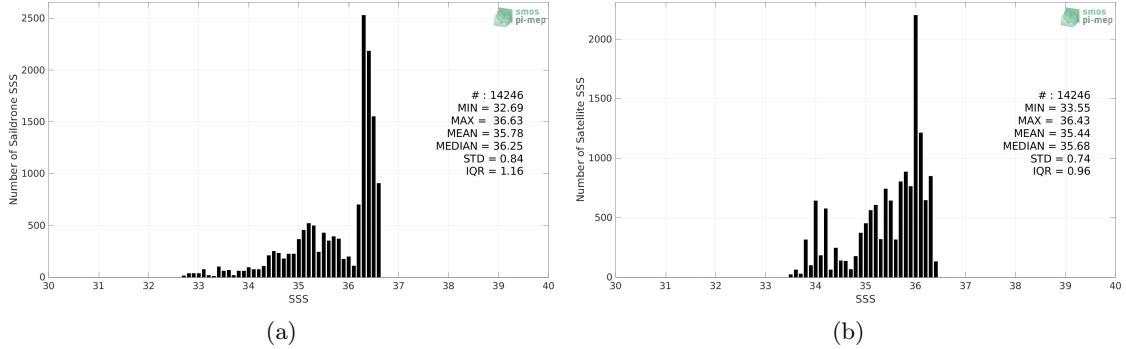
Figure 2: Histograms of SSS from Saildrone (a) and SMAP SSS L4 OI v2 - 7 Days (ESR) (b) considering all match-up pairs per bins of 0.1 over the Gulf of Mexico Pi-MEP region and for the full satellite product period.
