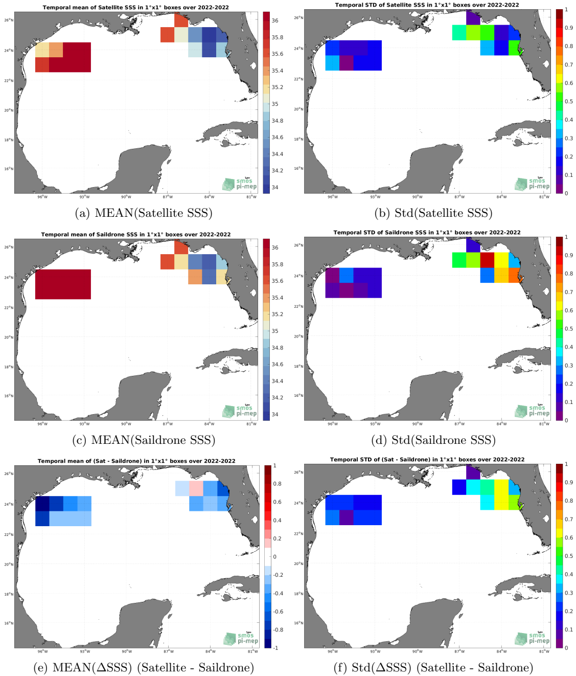
Figure 6: Temporal mean (left) and Std (right) of SSS from SMAP SSS L4 OI v2 - 7 Days (ESR) (top), Saildrone (middle), and of \Delta SSS (Satellite - Saildrone). Only match-up pairs are used to generate these maps.
