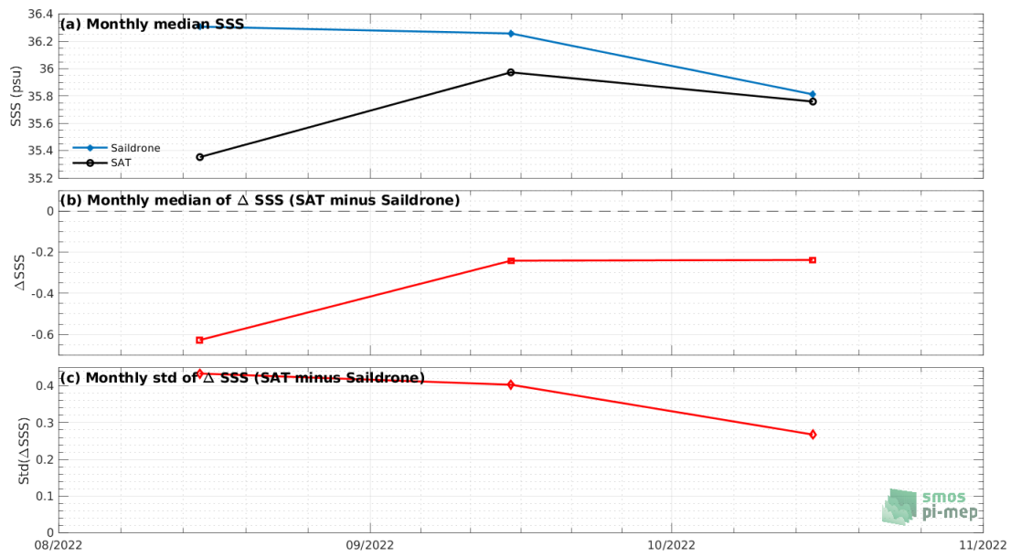
Figure 7: Time series of the monthly median SSS (top), median of \Delta SSS (Satellite - Sairdrone) and Std of \Delta SSS (Satellite - Sairdrone) over the Gulf of Mexico Pi-MEP region considering all match-ups collected by the Pi-MEP.
