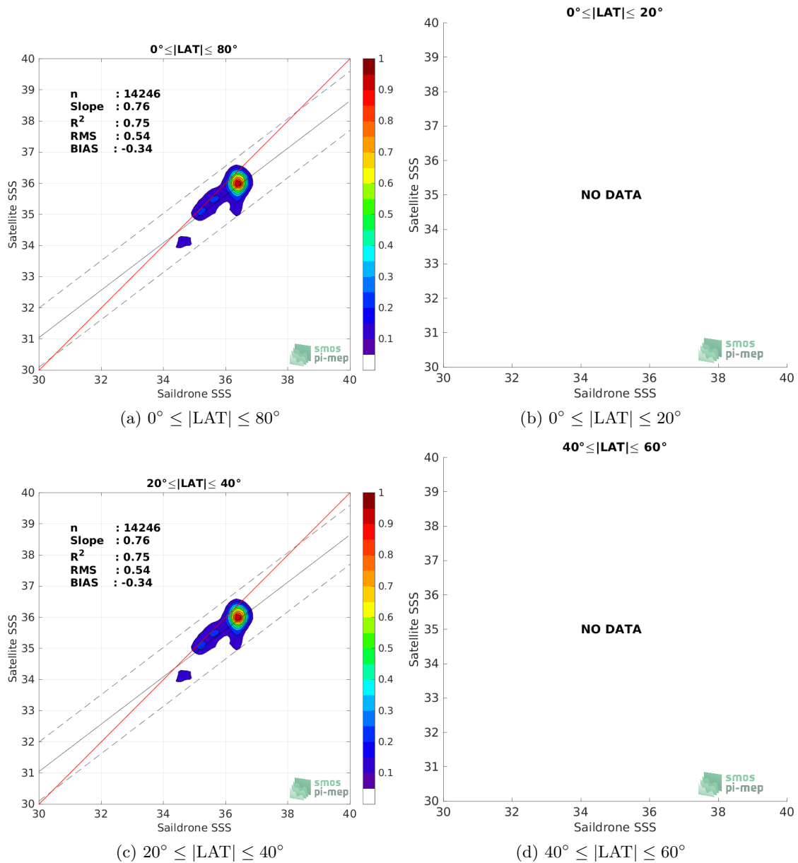
Figure 9: Contour maps of the concentration of SMAP SSS L4 OI v2 - 7 Days (ESR) SSS (y-axis) versus Saïldrone SSS (x-axis) at match-up pairs for different latitude bands. For each plot, the red line shows x=y . The black thin and dashed lines indicate a linear fit through the data cloud and the \pm 95\% confidence levels, respectively. The number match-up pairs n , the slope and R^2 coefficient of the linear fit, the root mean square (RMS) and the mean bias between satellite and in situ data are indicated for each latitude band in each plots.
