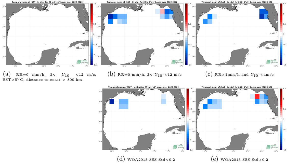
Figure 12: Temporal mean gridded over spatial boxes of size 1^{\circ}\times 1^{\circ} of \Delta\text{SSS} (SMAP SSS L4 OI v2 - 7 Days (ESR) - Saildrone) for 5 different subdatasets corresponding to:RR=0 mm/h, 3 < U_{10} < 12 m/s, SST >5^{\circ}\text{C} , distance to coast > 800 km (a), RR=0 mm/h, 3 < U_{10} < 12 m/s (b), RR >1 mm/h and U_{10} < 4 m/s (c), WOA2013 SSS Std <0.2 (d), WOA2013 SSS Std >0.2 (e).
