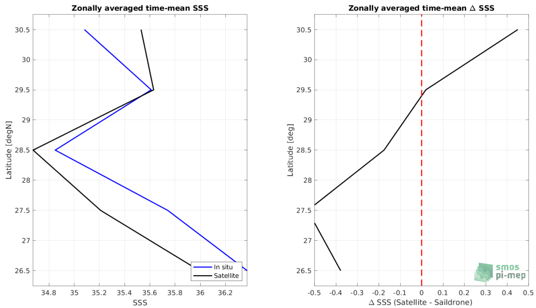
Figure 8: Left panel: Zonal mean SSS from SMAP SSS L4 OI v2 - 7 Days (ESR) satellite product (black) and from Sairdrone (blue). Right panel: Zonal mean of \Delta SSS (Satellite - Sairdrone) for all the collected Pi-MEP match-up pairs estimated over the full satellite product period.
