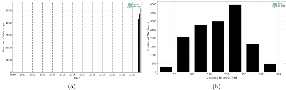
Figure 1: Number of match-ups between Saildrone and SMAP SSS L4 OI v2 - 7 Days (ESR) SSS as a function of time (a) and as function of the distance to coast (b) over the Gulf of Mexico Pi-MEP region and for the full satellite product period.
