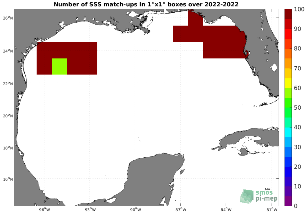
Figure 4: Number of SSS match-ups between Saildrone SSS and the SMAP SSS L4 OI v2 - 7 Days (ESR) SSS product for the Gulf of Mexico Pi-MEP region over 1^\circ \times 1^\circ boxes and for the full satellite product period.
