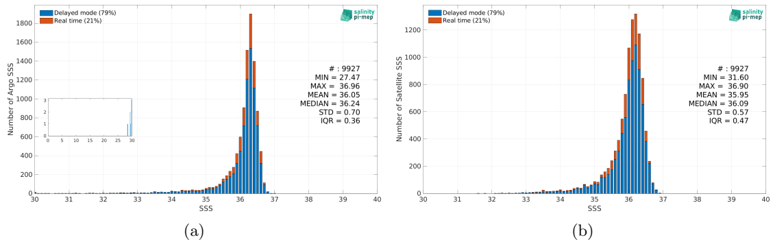
Figure 2: Histograms of SSS from Argo (a) and SMAP SSS L4 OI v2 - 7 Days (ESR) (b) considering all match-up pairs per bins of 0.1 over the Gulf of Mexico Pi-MEP region and for the full satellite product period.
