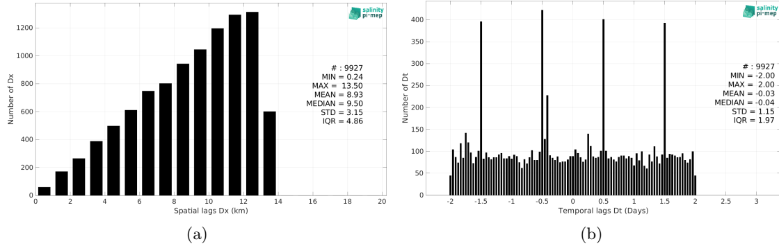
Figure 5: Histograms of the spatial (a) and temporal (b) lags between the location/time of the Argo measurement and the date of the corresponding SMAP SSS L4 OI v2 - 7 Days (ESR) SSS pixel.
