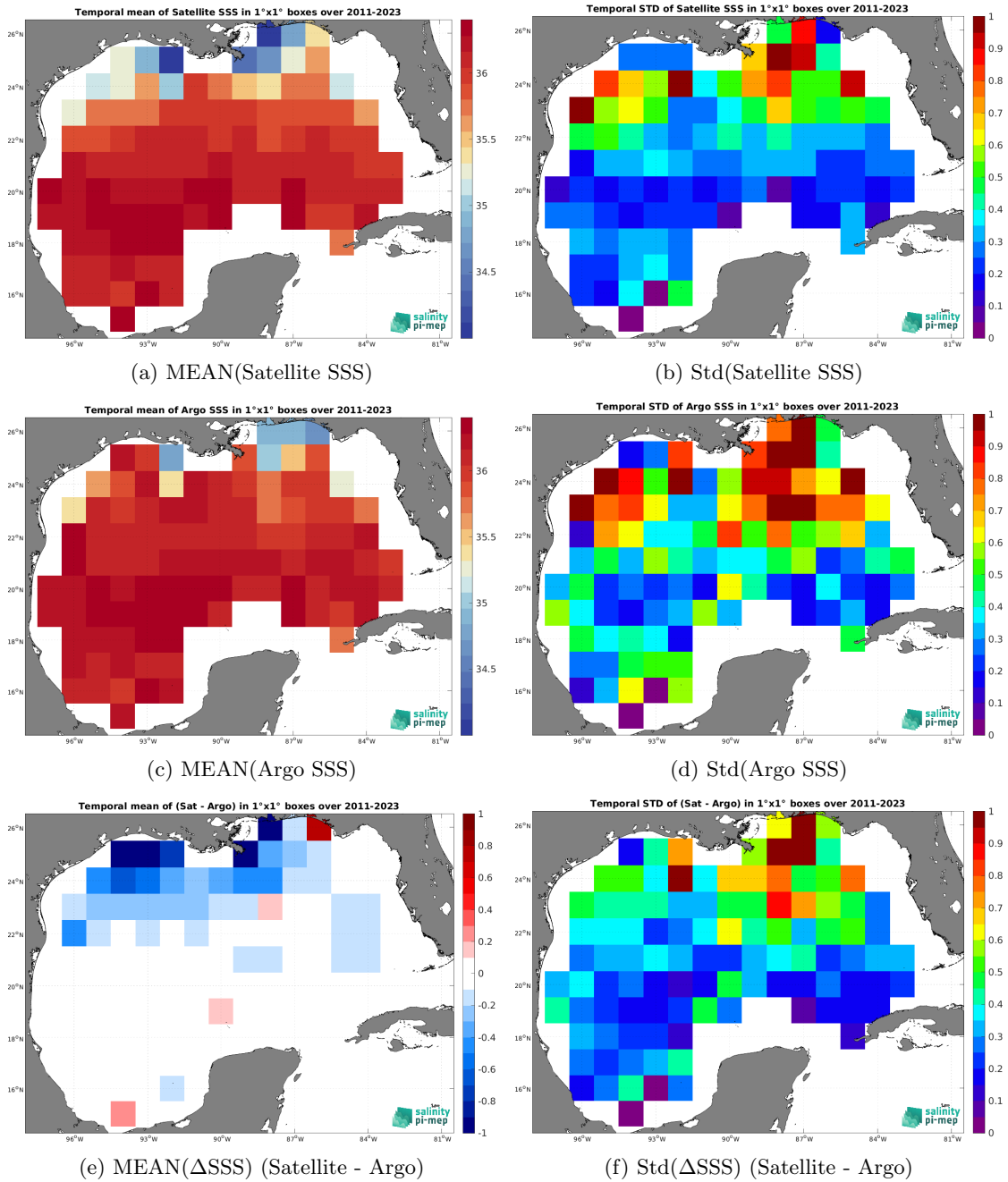
Figure 6: Temporal mean (left) and Std (right) of SSS from SMAP SSS L4 OI v2 - 7 Days (ESR) (top), Argo (middle), and of \Delta SSS (Satellite - Argo). Only match-up pairs are used to generate these maps.
