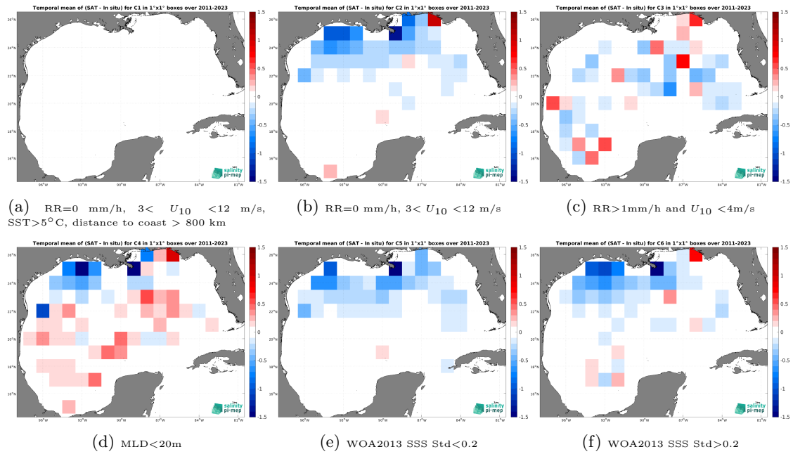
Figure 12: Temporal mean gridded over spatial boxes of size 1^\circ \times 1^\circ of \Delta SSS (SMAP SSS L4 OI v2 - 7 Days (ESR) - Argo) for 6 different subdatasets corresponding to:RR=0 mm/h, 3 < U_{10} < 12 m/s, SST >5^\circ C, distance to coast > 800 km (a), RR=0 mm/h, 3 < U_{10} < 12 m/s (b), RR >1 mm/h and U_{10} < 4 m/s (c),MLD <20 m (d),WOA2013 SSS Std <0.2 (e),WOA2013 SSS Std >0.2 (f).
