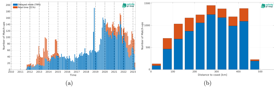
Figure 1: Number of match-ups between Argo and SMAP SSS L4 OI v2 - 7 Days (ESR) SSS as a function of time (a) and as function of the distance to coast (b) over the Gulf of Mexico Pi-MEP region and for the full satellite product period.
