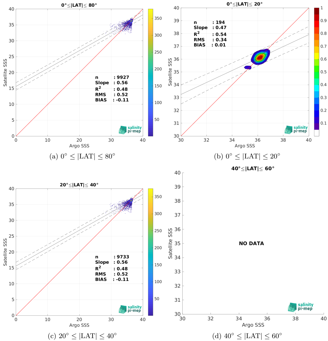
Figure 9: Contour maps of the concentration of SMAP SSS L4 OI v2 - 7 Days (ESR) SSS (y-axis) versus Argo SSS (x-axis) at match-up pairs for different latitude bands. For each plot, the red line shows x=y . The black thin and dashed lines indicate a linear fit through the data cloud and the \pm 95\% confidence levels, respectively. The number match-up pairs n , the slope and R^2 coefficient of the linear fit, the root mean square (RMS) and the mean bias between satellite and in situ data are indicated for each latitude band in each plots.
