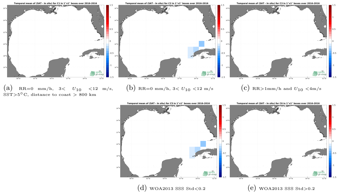
Figure 12: Temporal mean gridded over spatial boxes of size 1^{\circ}\times 1^{\circ} of \Delta\text{SSS} (SMAP SSS L4 OI v2 - Monthly (IPRC) - TSG (LEGOS-DM)) for 5 different subdatasets corresponding to:RR=0 mm/h, 3 < U_{10} < 12 m/s, SST >5^{\circ}\text{C} , distance to coast > 800 km (a), RR=0 mm/h, 3 < U_{10} < 12 m/s (b), RR >1 mm/h and U_{10} < 4 m/s (c), WOA2013 SSS Std <0.2 (d), WOA2013 SSS Std >0.2 (e).
