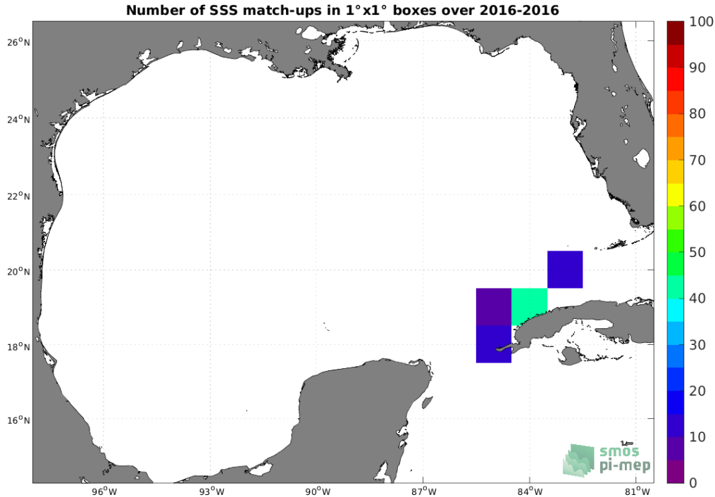
Figure 4: Number of SSS match-ups between TSG (LEGOS-DM) SSS and the SMAP SSS L4 OI v2 - Monthly (IPRC) SSS product for the Gulf of Mexico Pi-MEP region over 1^\circ \times 1^\circ boxes and for the full satellite product period.
