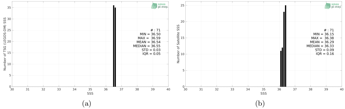
Figure 2: Histograms of SSS from TSG (LEGOS-DM) (a) and SMAP SSS L4 OI v2 - Monthly (IPRC) (b) considering all match-up pairs per bins of 0.1 over the Gulf of Mexico Pi-MEP region and for the full satellite product period.
