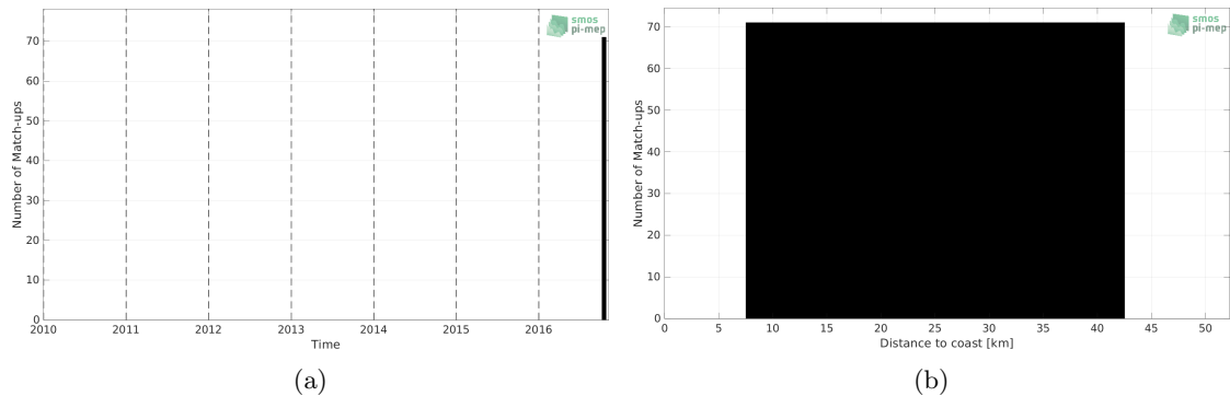
Figure 1: Number of match-ups between TSG (LEGOS-DM) and SMAP SSS L4 OI v2 - Monthly (IPRC) SSS as a function of time (a) and as function of the distance to coast (b) over the Gulf of Mexico Pi-MEP region and for the full satellite product period.
