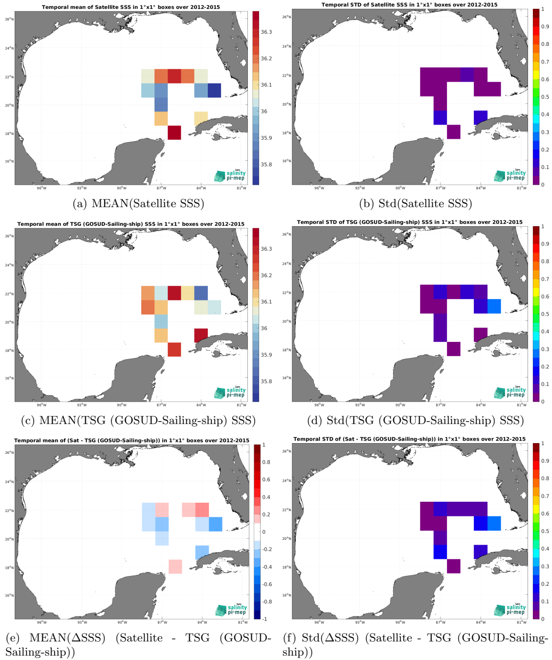
Figure 6: Temporal mean (left) and Std (right) of SSS from SMAP SSS L4 OI v2 - Monthly (IPRC) (top), TSG (GOSUD-Sailing-ship) (middle), and of \Delta SSS (Satellite - TSG (GOSUD-Sailing-ship)). Only match-up pairs are used to generate these maps.
