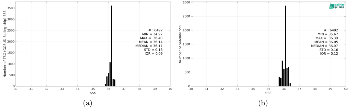
Figure 2: Histograms of SSS from TSG (GOSUD-Sailing-ship) (a) and SMAP SSS L4 OI v2 - Monthly (IPRC) (b) considering all match-up pairs per bins of 0.1 over the Gulf of Mexico Pi-MEP region and for the full satellite product period.
