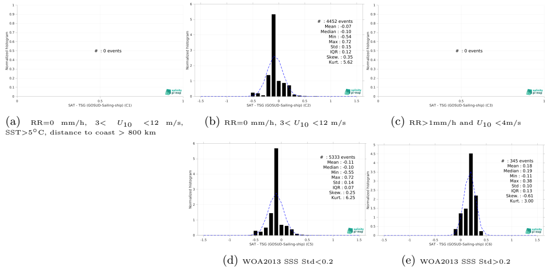
Figure 13: Normalized histogram of \Delta\text{SSS} (SMAP SSS L4 OI v2 - Monthly (IPRC) - TSG (GOSUD-Sailing-ship)) for 5 different subdatasets corresponding to: RR=0 mm/h, 3 < U_{10} < 12 m/s, SST > 5^{\circ}\text{C} , distance to coast > 800 km (a), RR=0 mm/h, 3 < U_{10} < 12 m/s (b), RR > 1\text{mm/h} and U_{10} < 4\text{m/s} (c), WOA2013 SSS Std < 0.2 (d), WOA2013 SSS Std > 0.2 (e).
