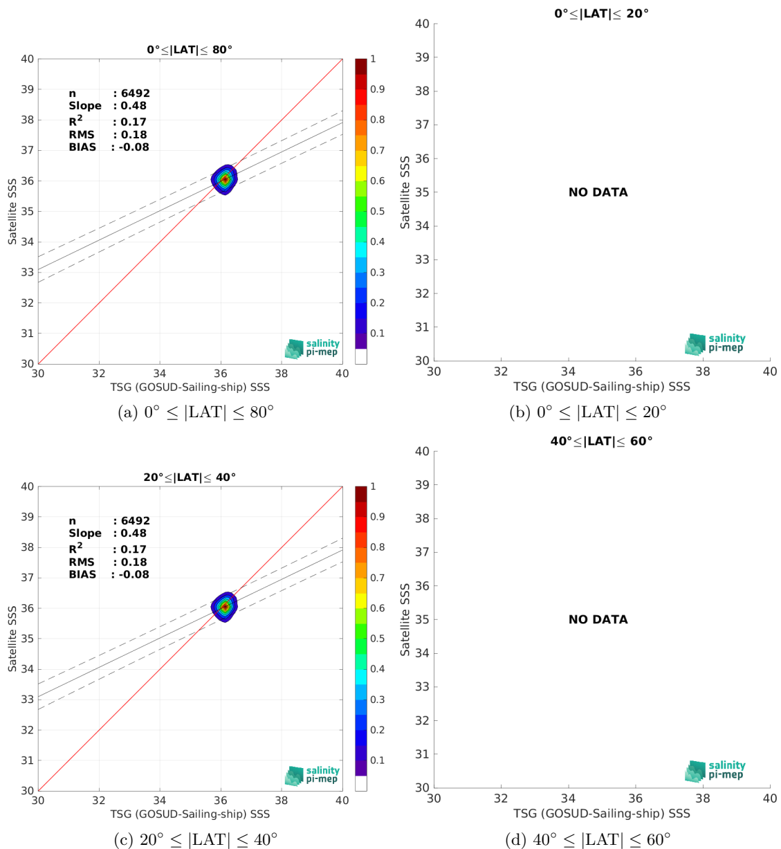
Figure 9: Contour maps of the concentration of SMAP SSS L4 OI v2 - Monthly (IPRC) SSS (y-axis) versus TSG (GOSUD-Sailing-ship) SSS (x-axis) at match-up pairs for different latitude bands. For each plot, the red line shows x=y . The black thin and dashed lines indicate a linear fit through the data cloud and the \pm 95\% confidence levels, respectively. The number match-up pairs n , the slope and R^2 coefficient of the linear fit, the root mean square (RMS) and the mean bias between satellite and in situ data are indicated for each latitude band in each plots.
