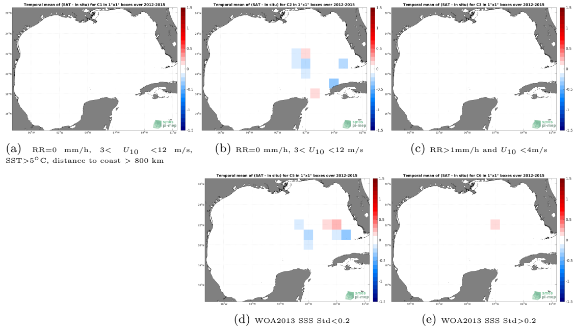
Figure 12: Temporal mean gridded over spatial boxes of size 1^\circ \times 1^\circ of \Delta SSS (SMAP SSS L4 OI v2 - Monthly (IPRC) - TSG (GOSUD-Sailing-ship)) for 5 different subdatasets corresponding to:RR=0 mm/h, 3 < U_{10} < 12 m/s, SST >5^\circ\text{C} , distance to coast > 800 km (a), RR=0 mm/h, 3 < U_{10} < 12 m/s (b), RR >1 mm/h and U_{10} < 4 m/s (c), WOA2013 SSS Std <0.2 (d), WOA2013 SSS Std >0.2 (e).
