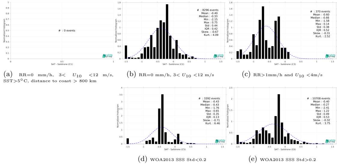
Figure 13: Normalized histogram of \Delta SSS (SMAP SSS L4 OI v2 - Monthly (IPRC) - Saikdrone) for 5 different subdatasets corresponding to: RR=0 mm/h, 3 < U_{10} < 12 m/s, SST > 5°C, distance to coast > 800 km (a), RR=0 mm/h, 3 < U_{10} < 12 m/s (b), RR > 1mm/h and U_{10} < 4 m/s (c), WOA2013 SSS Std < 0.2 (d), WOA2013 SSS Std > 0.2 (e).
