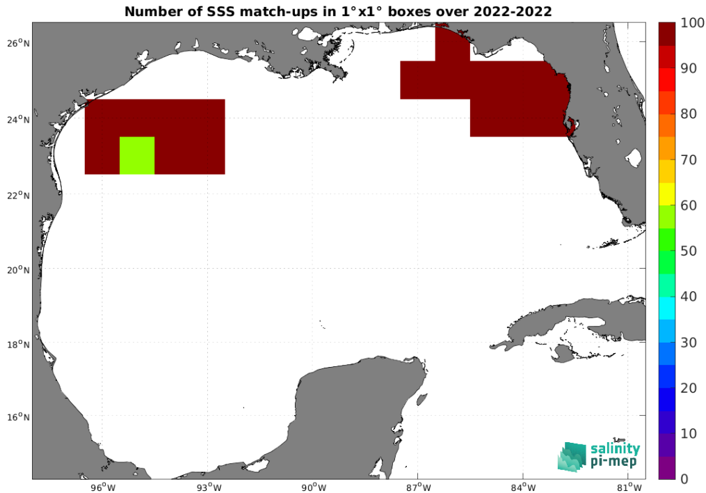
Figure 4: Number of SSS match-ups between Saildrone SSS and the SMAP SSS L4 OI v2 - Monthly (IPRC) SSS product for the Gulf of Mexico Pi-MEP region over 1^\circ \times 1^\circ boxes and for the full satellite product period.
