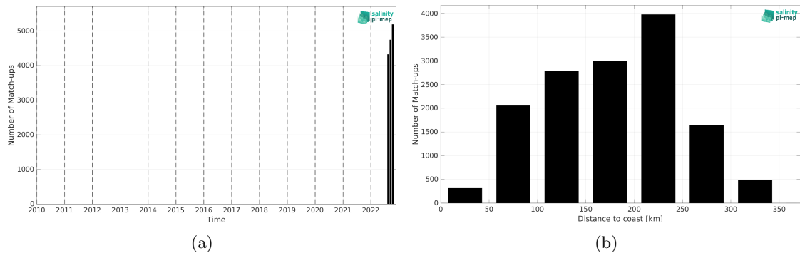
Figure 1: Number of match-ups between Saildrone and SMAP SSS L4 OI v2 - Monthly (IPRC) SSS as a function of time (a) and as function of the distance to coast (b) over the Gulf of Mexico Pi-MEP region and for the full satellite product period.
