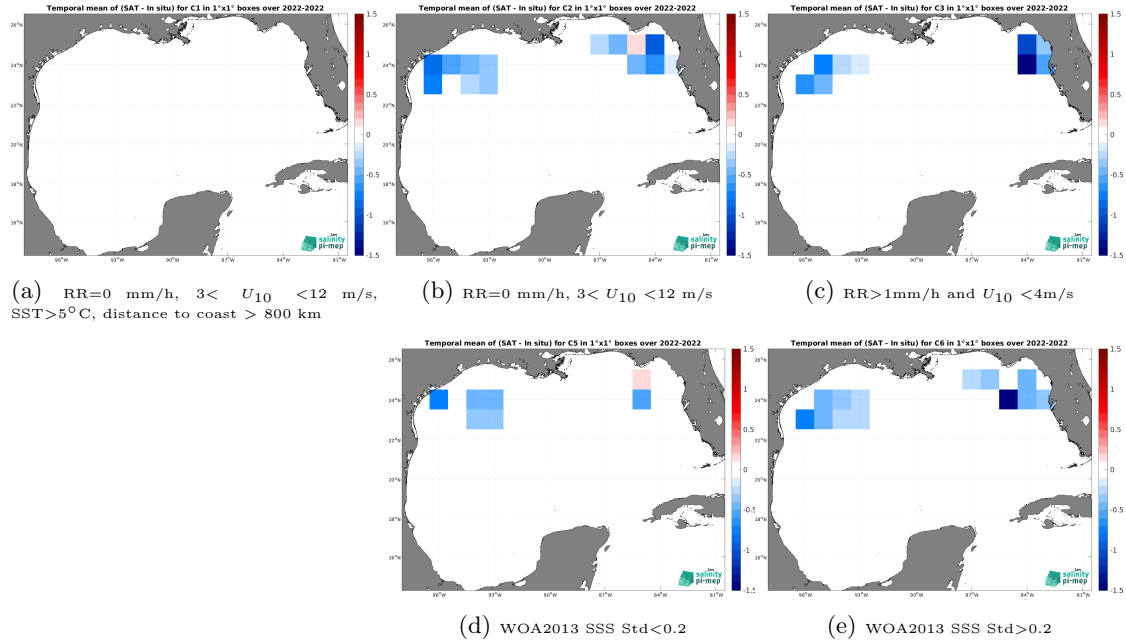
Figure 12: Temporal mean gridded over spatial boxes of size 1^{\circ}\times 1^{\circ} of \Delta\text{SSS} (SMAP SSS L4 OI v2 - Monthly (IPRC) - Saildrone) for 5 different subdatasets corresponding to:RR=0 mm/h, 3 < U_{10} < 12 m/s, SST >5^{\circ}\text{C} , distance to coast > 800 km (a), RR=0 mm/h, 3 < U_{10} < 12 m/s (b), RR >1 mm/h and U_{10} < 4 m/s (c), WOA2013 SSS Std <0.2 (d), WOA2013 SSS Std >0.2 (e).
