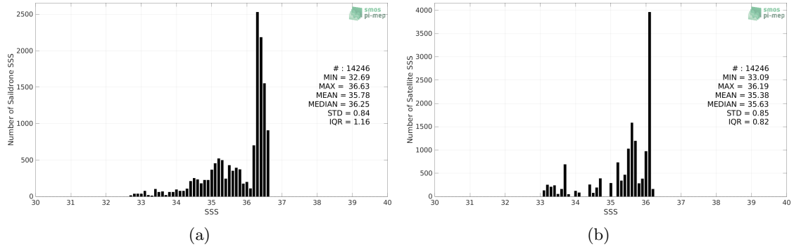
Figure 2: Histograms of SSS from Sairdrone (a) and SMAP SSS L4 OI v2 - Monthly (IPRC) (b) considering all match-up pairs per bins of 0.1 over the Gulf of Mexico Pi-MEP region and for the full satellite product period.
