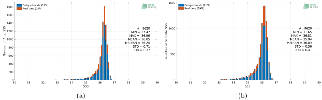
Figure 2: Histograms of SSS from Argo (a) and SMAP SSS L4 OI v2 - Monthly (IPRC) (b) considering all match-up pairs per bins of 0.1 over the Gulf of Mexico Pi-MEP region and for the full satellite product period.
