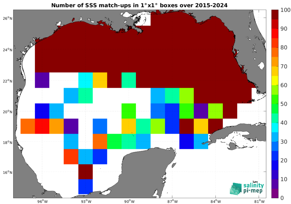
Figure 5: Number of SSS match-ups between TSG (SAMOS) SSS and the SMAP SSS L3 v6 - 8-Day running (RSS) SSS product for the Gulf of Mexico Pi-MEP region over 1^\circ \times 1^\circ boxes and for the full satellite product period.
