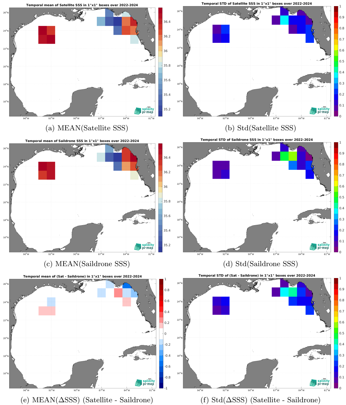
Figure 7: Temporal mean (left) and Std (right) of SSS from SMAP SSS L3 v6 - 8-Day running (RSS) (top), Saildrone (middle), and of \Delta SSS (Satellite - Saildrone). Only match-up pairs are used to generate these maps.
