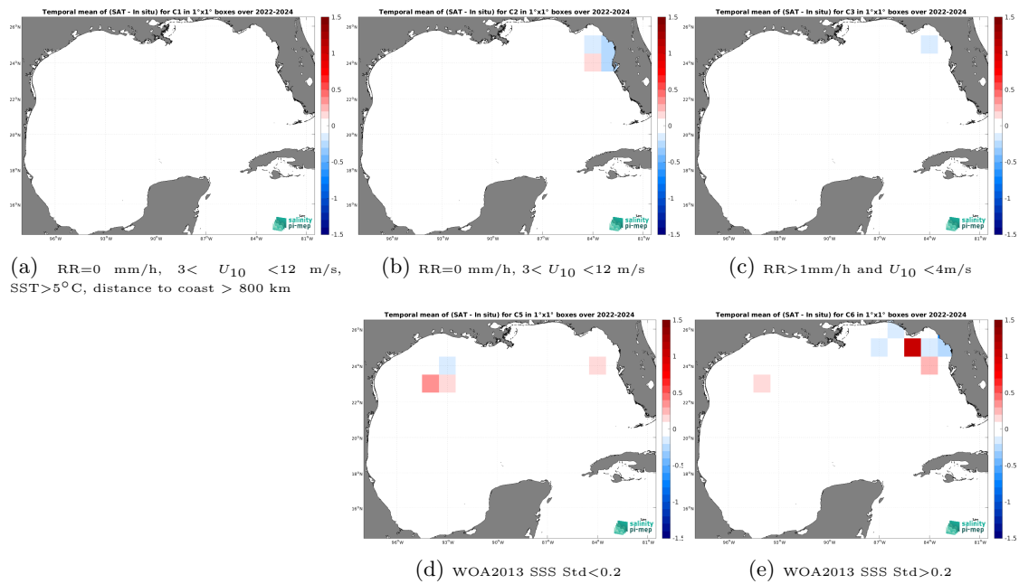
Figure 14: Temporal mean gridded over spatial boxes of size 1^\circ \times 1^\circ of \Delta\text{SSS} (SMAP SSS L3 v6 - 8-Day running (RSS) - Sairdrone) for 5 different subdatasets corresponding to:RR=0 mm/h, 3 < U_{10} < 12 m/s, SST>5°C, distance to coast > 800 km (a), RR=0 mm/h, 3 < U_{10} < 12 m/s (b), RR>1mm/h and U_{10} < 4 m/s (c), WOA2013 SSS Std<0.2 (d), WOA2013 SSS Std>0.2 (e).
