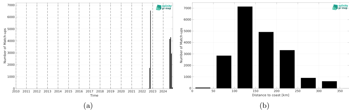
Figure 2: Number of match-ups between Saildrone and SMAP SSS L3 v6 - 8-Day running (RSS) SSS as a function of time (a) and as function of the distance to coast (b) over the Gulf of Mexico Pi-MEP region and for the full satellite product period.
