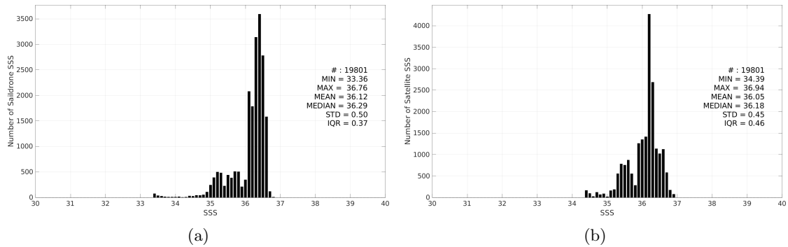
Figure 3: Histograms of SSS from Saildrone (a) and SMAP SSS L3 v6 - 8-Day running (RSS) (b) considering all match-up pairs per bins of 0.1 over the Gulf of Mexico Pi-MEP region and for the full satellite product period.
