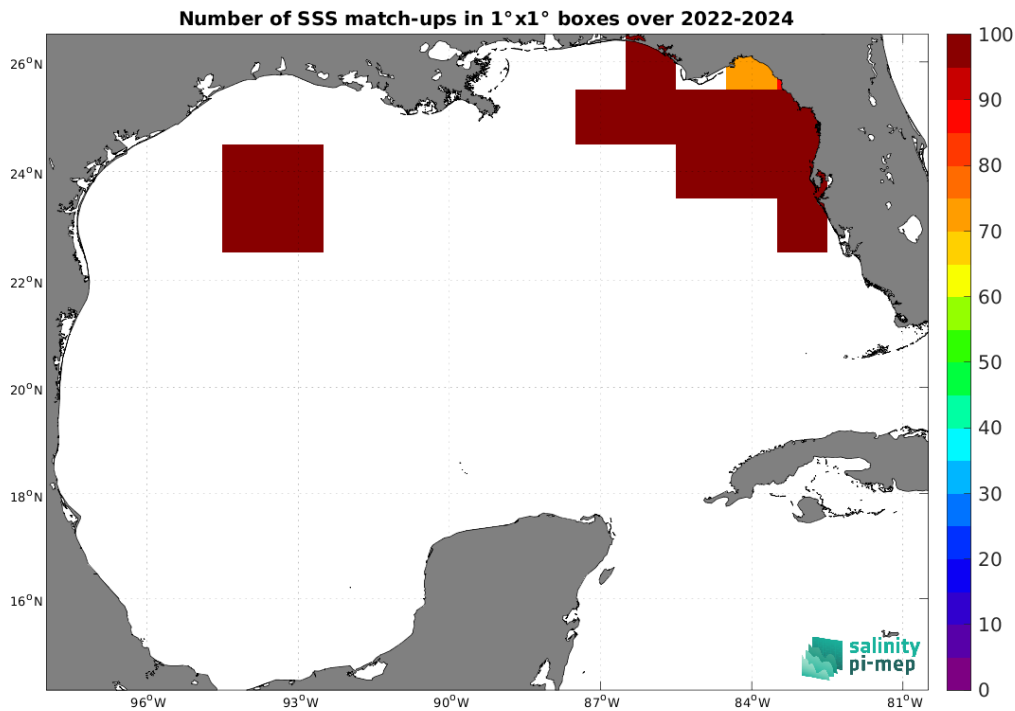
Figure 5: Number of SSS match-ups between Saildrone SSS and the SMAP SSS L3 v6 - 8-Day running (RSS) SSS product for the Gulf of Mexico Pi-MEP region over 1^\circ \times 1^\circ boxes and for the full satellite product period.
