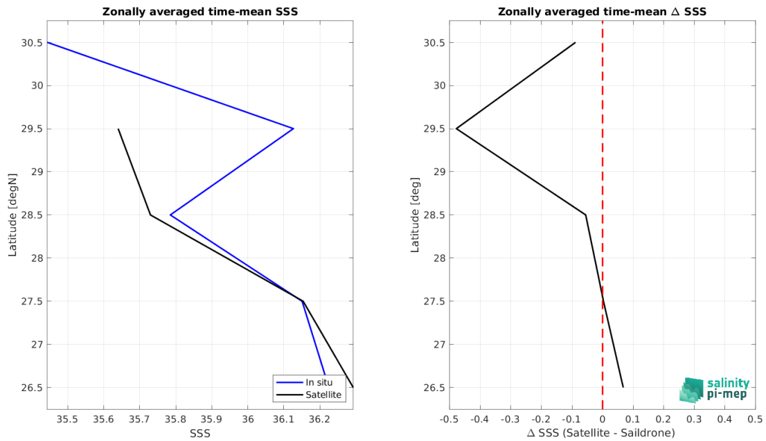
Figure 9: Left panel: Zonal mean SSS from SMAP SSS L3 v6 - 8-Day running (RSS) satellite product (black) and from Sairdrone (blue). Right panel: Zonal mean of \Delta SSS (Satellite - Sairdrone) for all the collected Pi-MEP match-up pairs estimated over the full satellite product period.
