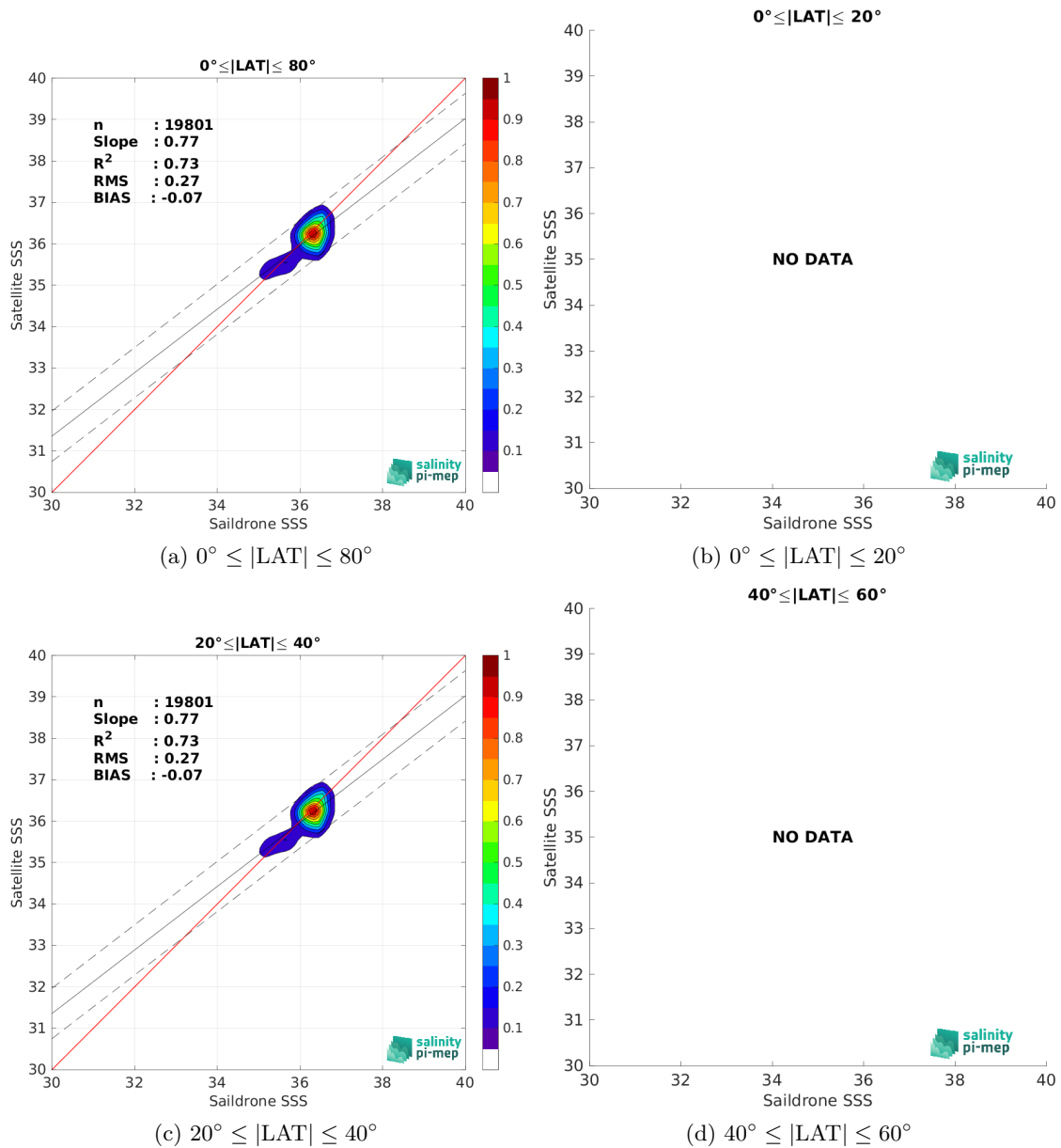
Figure 10: Contour maps of the concentration of SMAP SSS L3 v6 - 8-Day running (RSS) SSS (y-axis) versus Sailldrone SSS (x-axis) at match-up pairs for different latitude bands. For each plot, the red line shows x=y . The black thin and dashed lines indicate a linear fit through the data cloud and the \pm 95\% confidence levels, respectively. The number match-up pairs n , the slope and R^2 coefficient of the linear fit, the root mean square (RMS) and the mean bias between satellite and in situ data are indicated for each latitude band in each plots.
