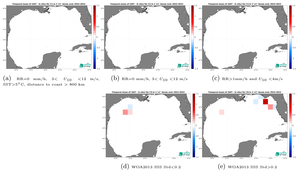
Figure 14: Temporal mean gridded over spatial boxes of size 1^\circ \times 1^\circ of \Delta SSS (SMAP SSS L3 v6 - 8-Day running (RSS) - Sairdrone) for 5 different subdatasets corresponding to: RR=0 mm/h, 3 < U_{10} < 12 m/s, SST > 5°C, distance to coast > 800 km (a), RR=0 mm/h, 3 < U_{10} < 12 m/s (b), RR > 1mm/h and U_{10} < 4 m/s (c), WOA2013 SSS Std < 0.2 (d), WOA2013 SSS Std > 0.2 (e).
