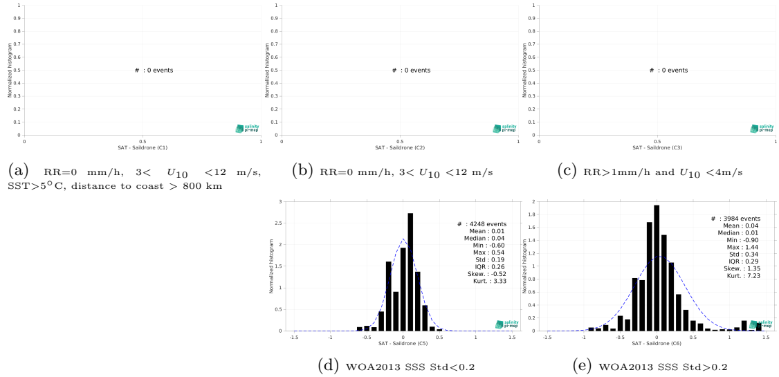
Figure 15: Normalized histogram of \Delta SSS (SMAP SSS L3 v6 - 8-Day running (RSS) - Sairdrone) for 5 different subdatasets corresponding to: RR=0 mm/h, 3 < U_{10} < 12 m/s, SST > 5°C, distance to coast > 800 km (a), RR=0 mm/h, 3 < U_{10} < 12 m/s (b), RR > 1mm/h and U_{10} < 4 m/s (c), WOA2013 SSS Std < 0.2 (d), WOA2013 SSS Std > 0.2 (e).
