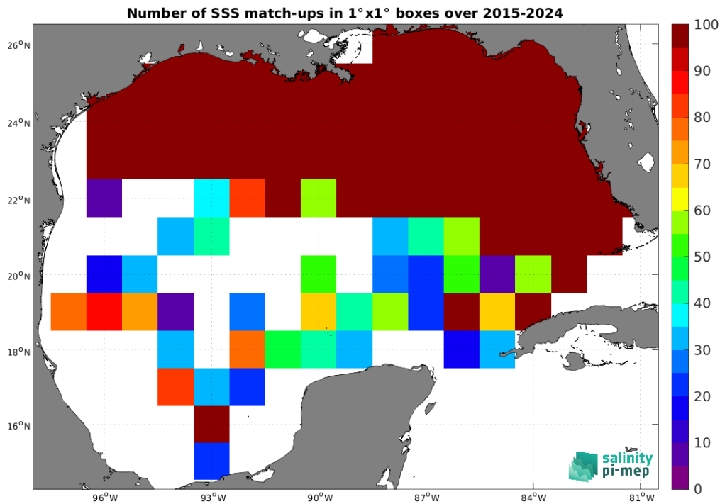
Figure 5: Number of SSS match-ups between TSG (SAMOS) SSS and the SMAP SSS L3 v6 - Monthly (RSS) SSS product for the Gulf of Mexico Pi-MEP region over 1^\circ \times 1^\circ boxes and for the full satellite product period.
