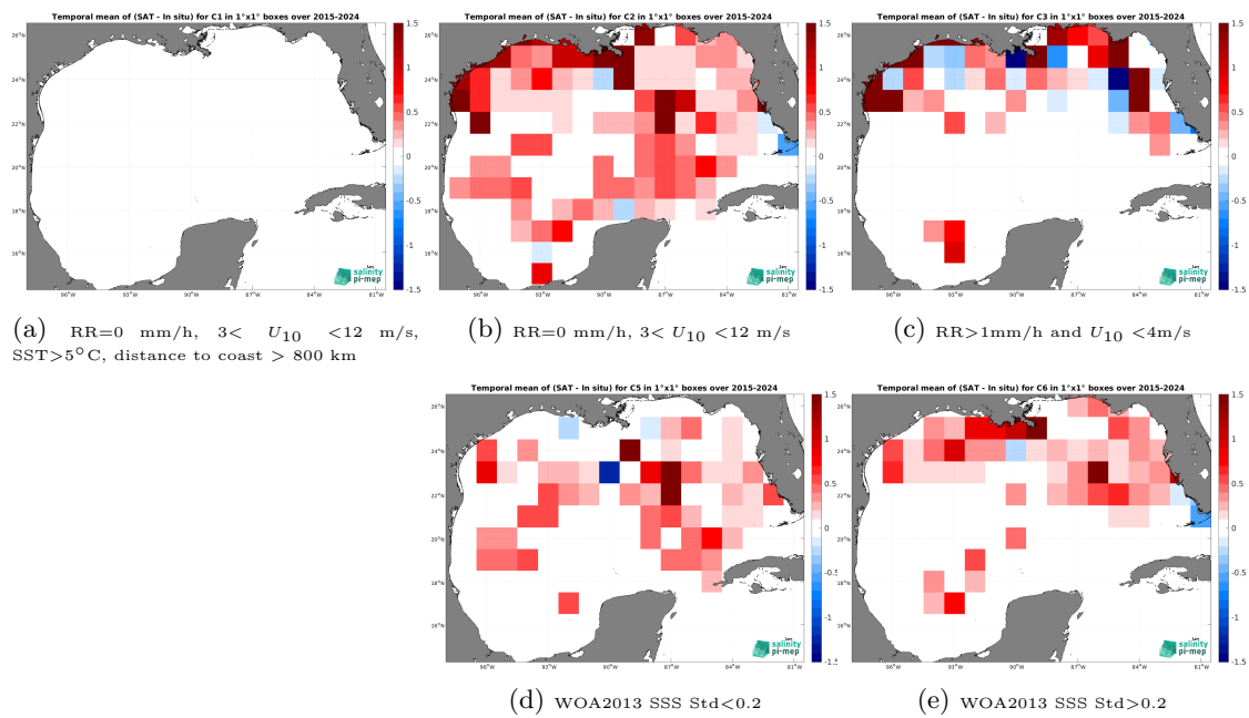
Figure 14: Temporal mean gridded over spatial boxes of size 1^\circ \times 1^\circ of \Delta SSS (SMAP SSS L3 v6 - Monthly (RSS) - TSG (SAMOS)) for 5 different subdatasets corresponding to:RR=0 mm/h, 3 < U_{10} < 12 m/s, SST >5^\circ\text{C} , distance to coast > 800 km (a), RR=0 mm/h, 3 < U_{10} < 12 m/s (b), RR >1 mm/h and U_{10} < 4 m/s (c), WOA2013 SSS Std <0.2 (d), WOA2013 SSS Std >0.2 (e).
