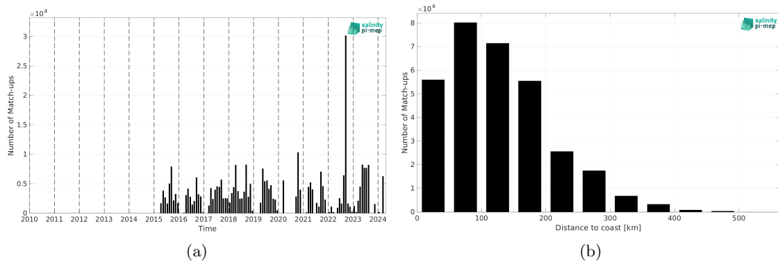
Figure 2: Number of match-ups between TSG (SAMOS) and SMAP SSS L3 v6 - Monthly (RSS) SSS as a function of time (a) and as function of the distance to coast (b) over the Gulf of Mexico Pi-MEP region and for the full satellite product period.
