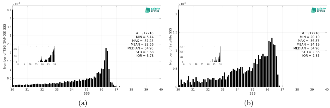
Figure 3: Histograms of SSS from TSG (SAMOS) (a) and SMAP SSS L3 v6 - Monthly (RSS) (b) considering all match-up pairs per bins of 0.1 over the Gulf of Mexico Pi-MEP region and for the full satellite product period.
