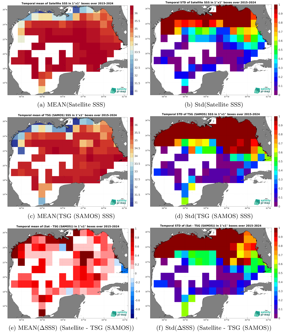
Figure 7: Temporal mean (left) and Std (right) of SSS from SMAP SSS L3 v6 - Monthly (RSS) (top), TSG (SAMOS) (middle), and of \Delta SSS (Satellite - TSG (SAMOS)). Only match-up pairs are used to generate these maps.
